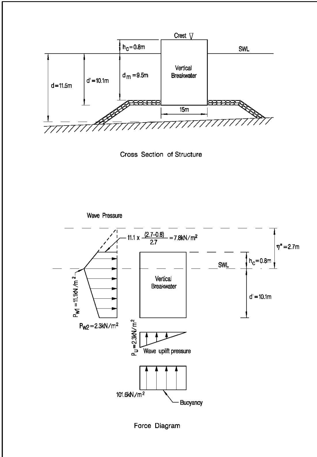
Figure C1 – Wave Force on Vertical Breakwater
