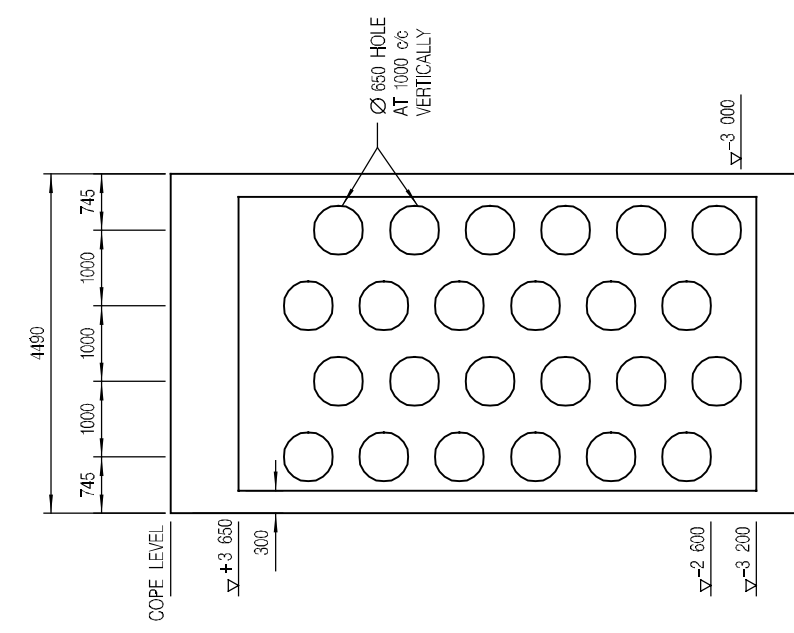
FRONT VIEW OF WAVE ABSORBING CHAMBER SCALE 1:100
