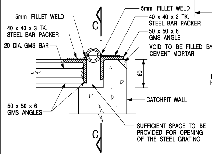
SECTIONAL ELEVATION (DETAIL 'C')
