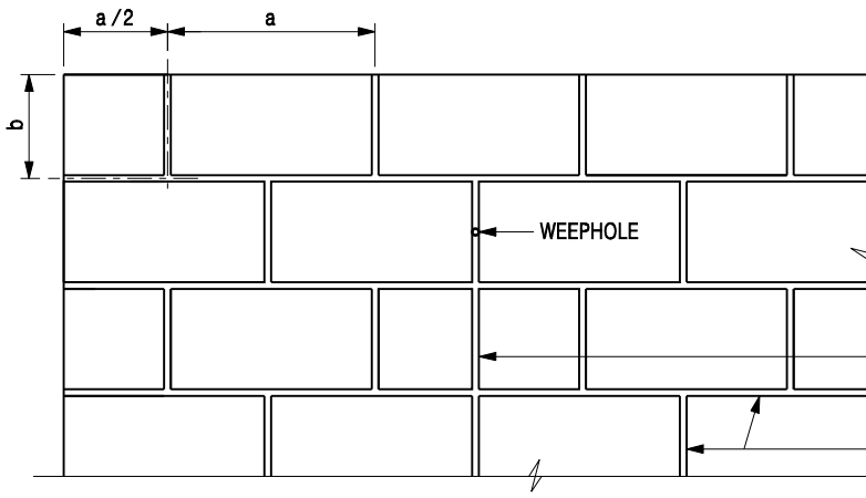
SMALL BLOCK PATTERN SCALE 1 : 25
