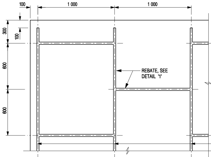
LARGE BLOCK PATTERN SCALE 1 : 25
