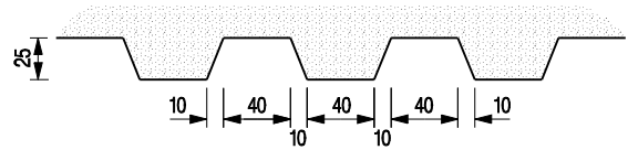
SHALLOW RIB PATTERN SCALE 1 : 5
