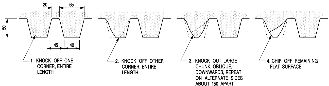
FRACTURED RIB FINISH SCALE 1 : 5
