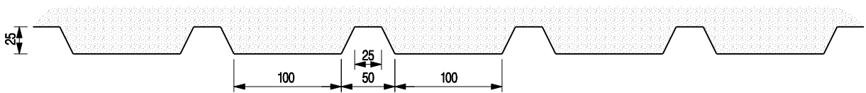
SHIP-LAP PATTERN SCALE 1 : 5
