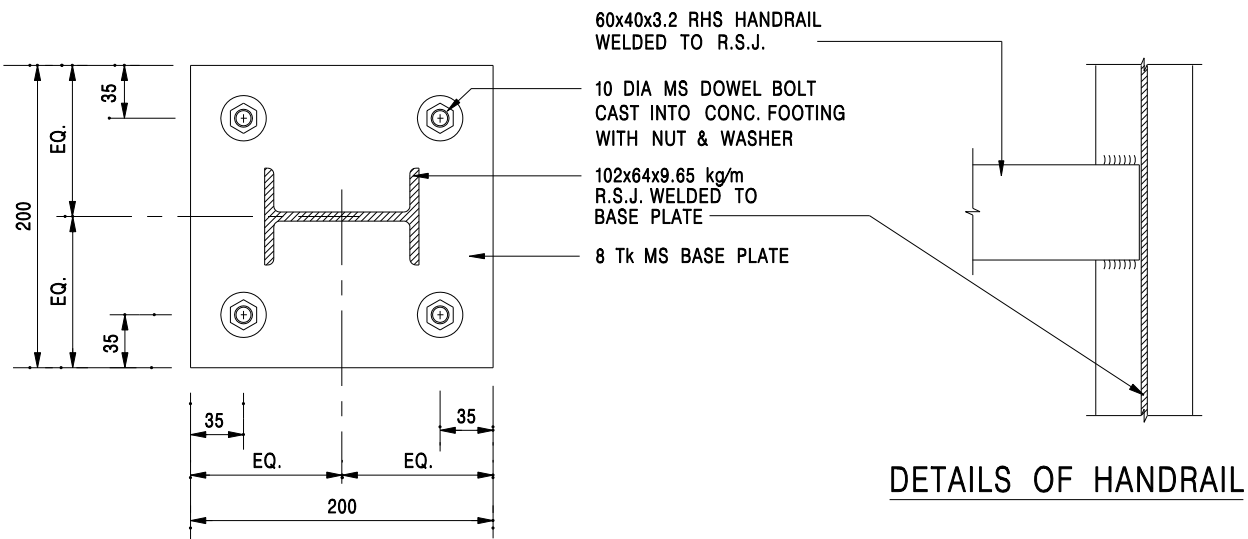
DETAILS OF BASE PLATE
