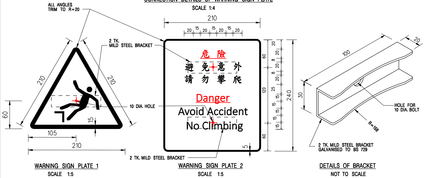
CONNECTION DETAILS OF WARNING SIGN PLATE
