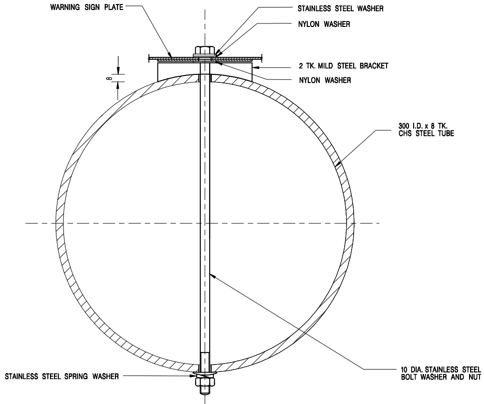
CONNECTION DETAILS OF WARNING SIGN PLATE
