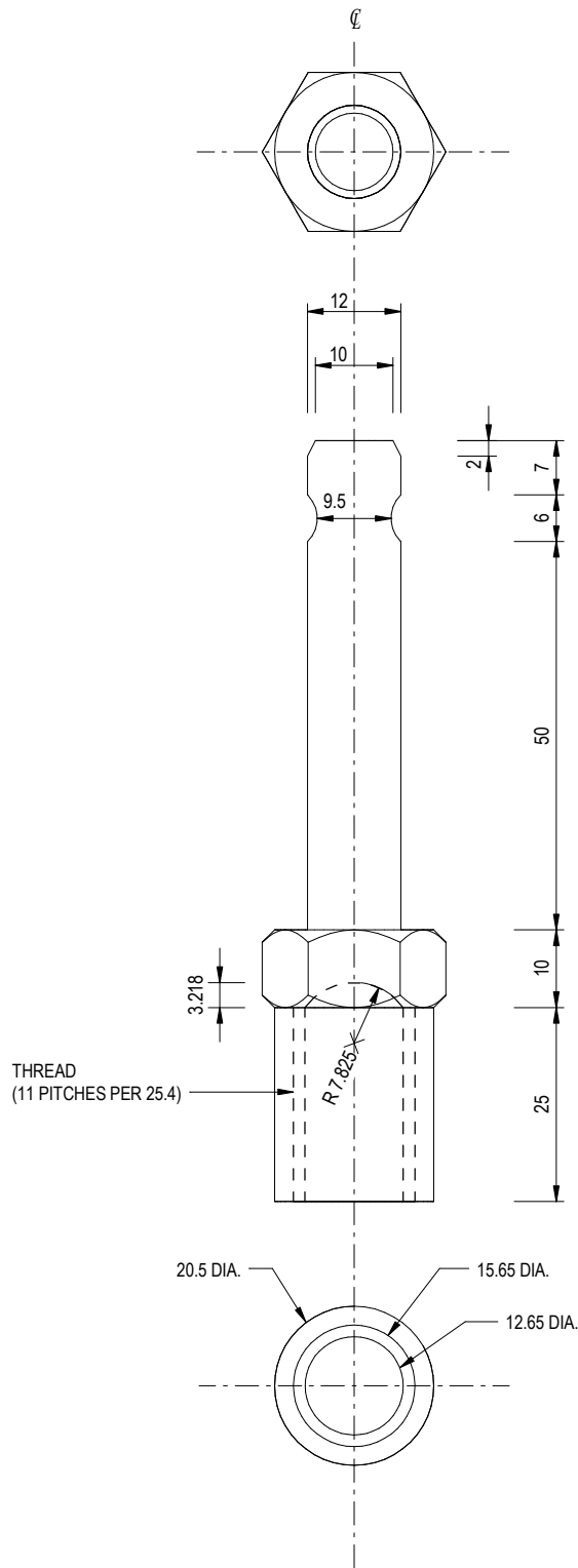
PRISM ADAPTOR
