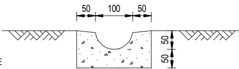
SECTION A - A (FOR SOIL SLOPE WITHOUT EROSION CONTROL MAT) SCALE 1 : 10
