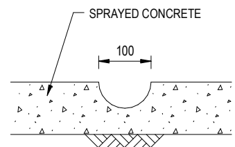
SECTION A - A (FOR SHOTCRETED SLOPE) SCALE 1 : 10
