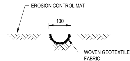
SECTION A - A (FOR SOIL SLOPE WITH EROSION CONTROL MAT) SCALE 1 : 10
