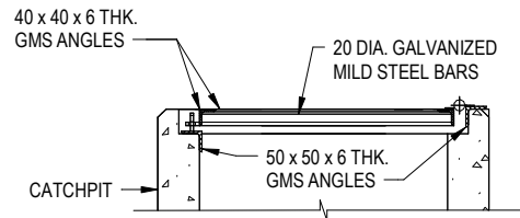
SECTIONAL ELEVATION
