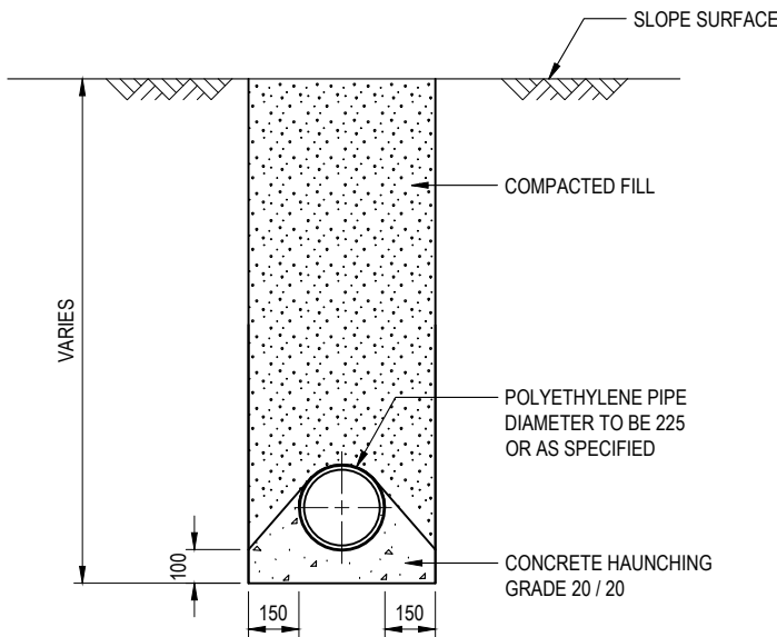
TYPICAL SECTION OF DRAIN FROM MANHOLE
