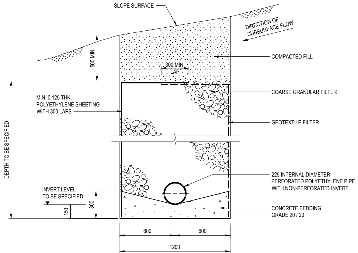
TYPICAL SECTION OF CUT-OFF DRAIN
