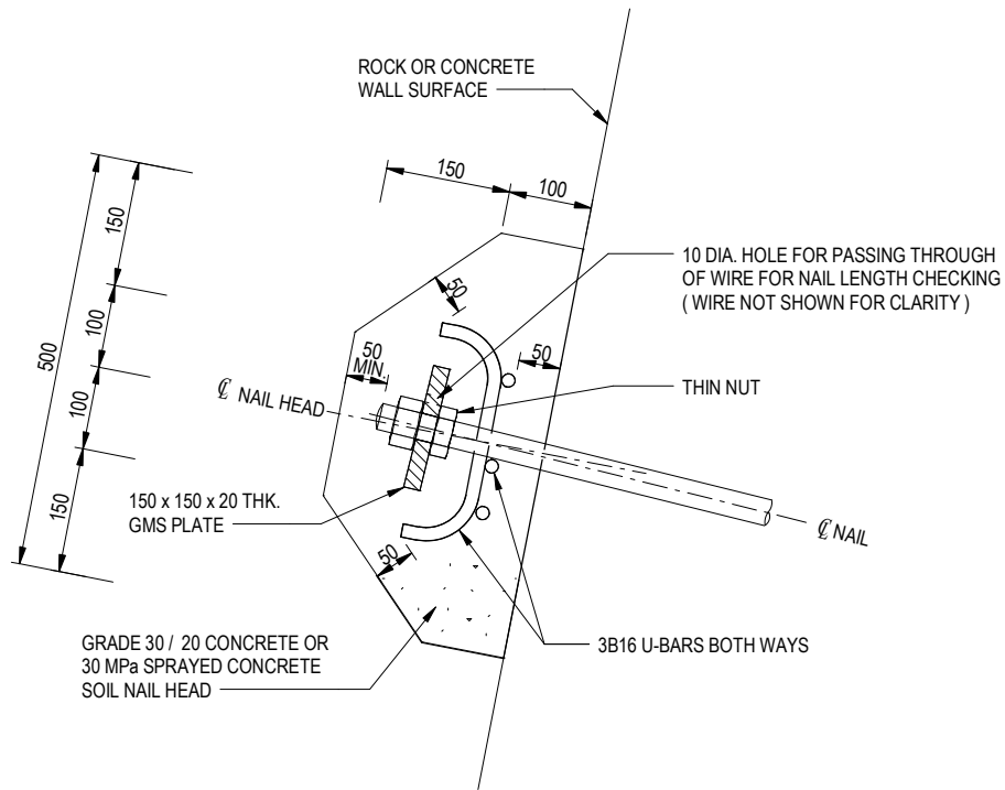
TYPICAL SECTION OF SOIL NAIL HEAD ON ROCK OR CONCRETE WALL SURFACE
