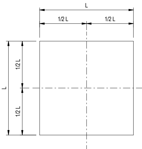
VIEW NORMAL TO SOIL NAIL HEAD
