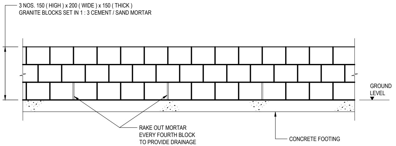
SECTIONAL ELEVATION A - A
