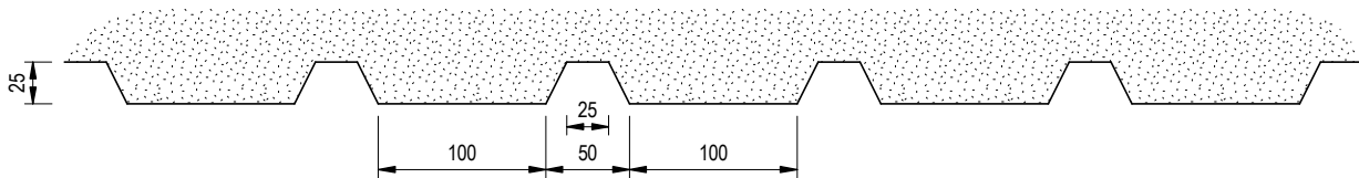
SHIP-LAP PATTERN SCALE 1:5
