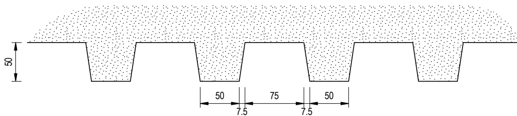
DEEP RIB PATTERN SCALE 1:5
