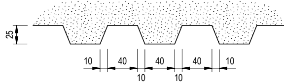
SHALLOW RIB PATTERN SCALE 1:5
