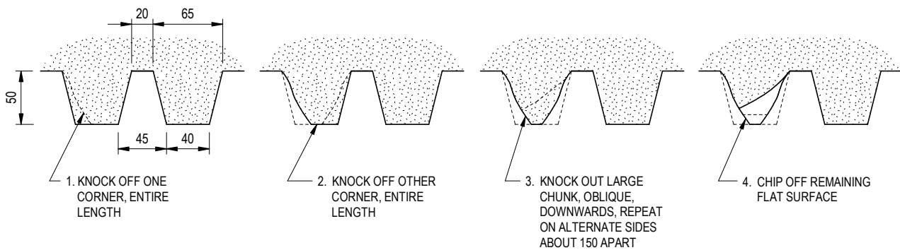
FRACTURED RIB FINISH SCALE 1:5
