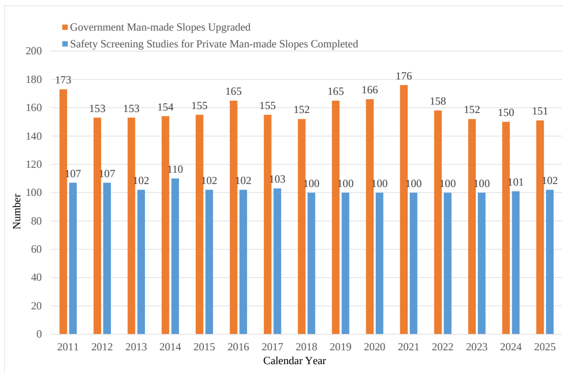
Figure 1 – Annual Outputs of Upgrading Works for Government Man-made Slopes and Safety-screening Studies for Private Man-made Slopes under the LPMitP from 2011 to 2025
