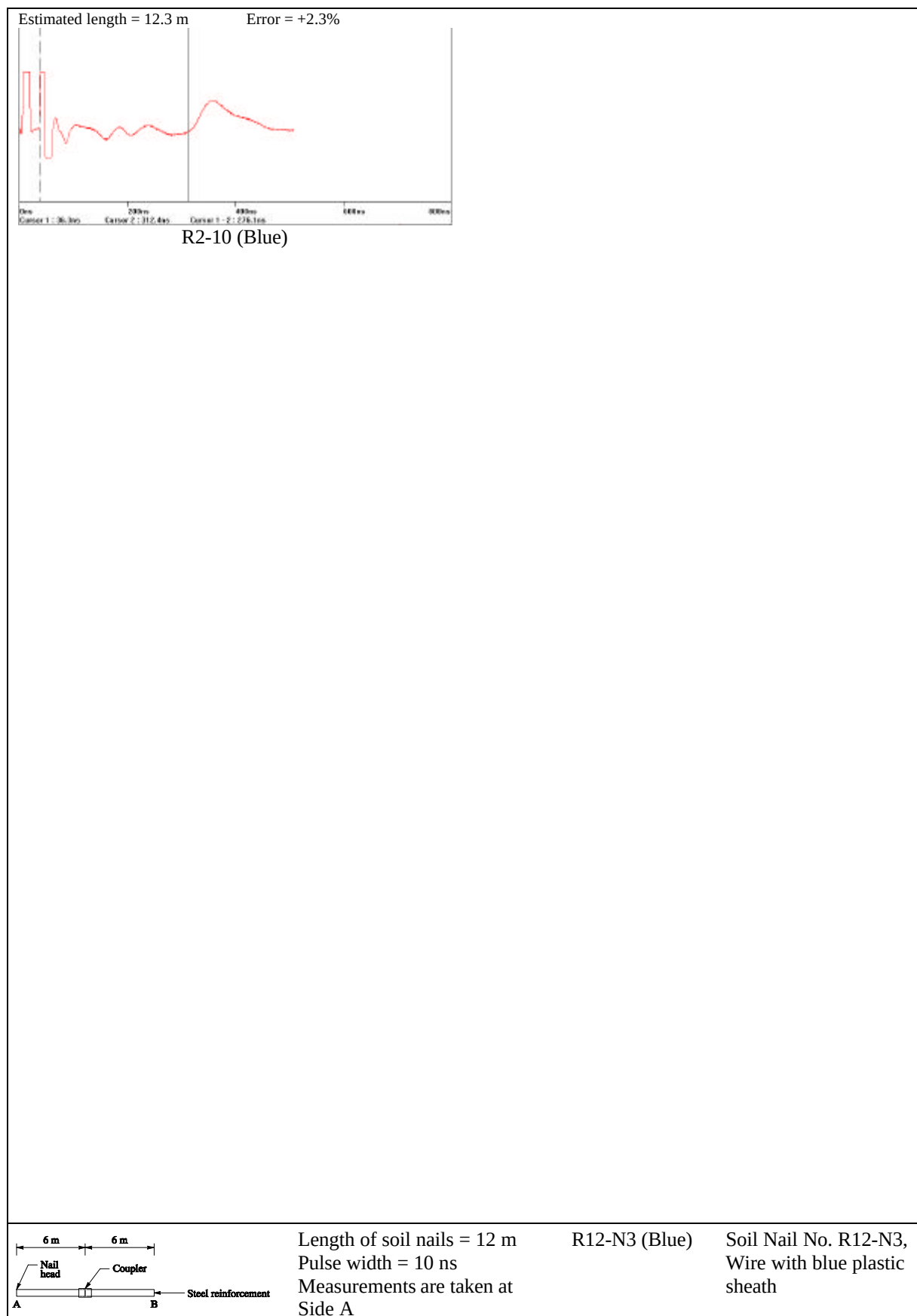
Figure 2 - TDR Test Results at an LPM Site along Tai Po Road
