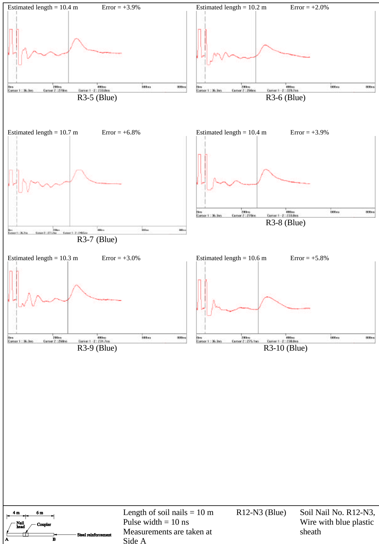
Figure 3 - TDR Test Results at an LPM Site along Tai Po Road
