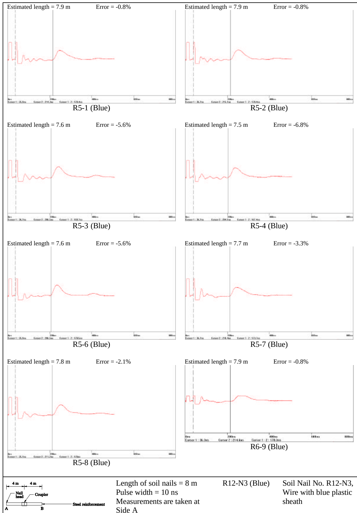
Figure 4 - TDR Test Results at an LPM Site along Tai Po Road
