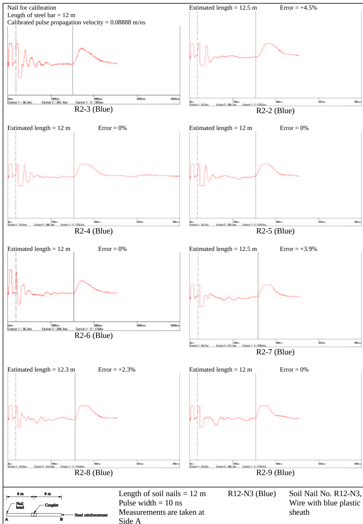
Figure 1 - TDR Test Results at an LPM Site along Tai Po Road
