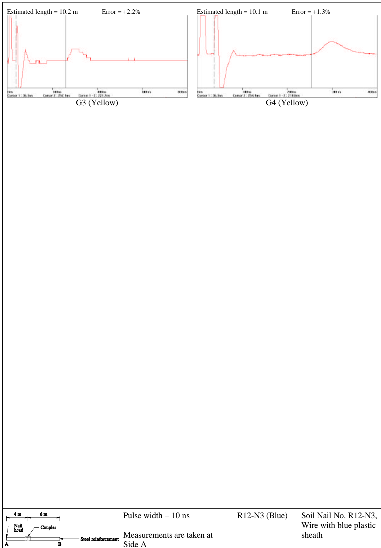
Figure 5 - TDR Test Results at an LPM Site in Chai Wan
