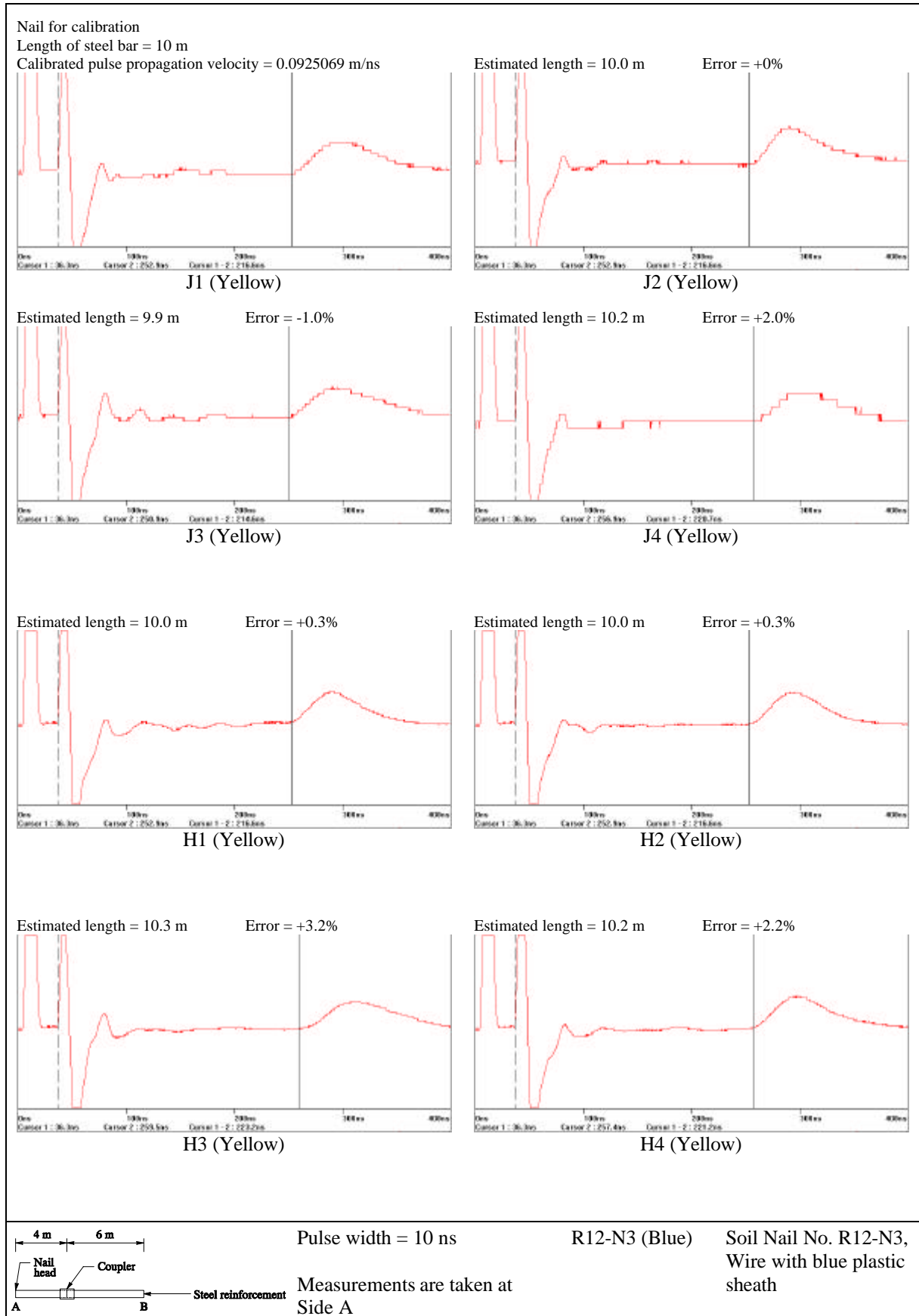
Figure 4 - TDR Test Results at an LPM Site in Chai Wan
