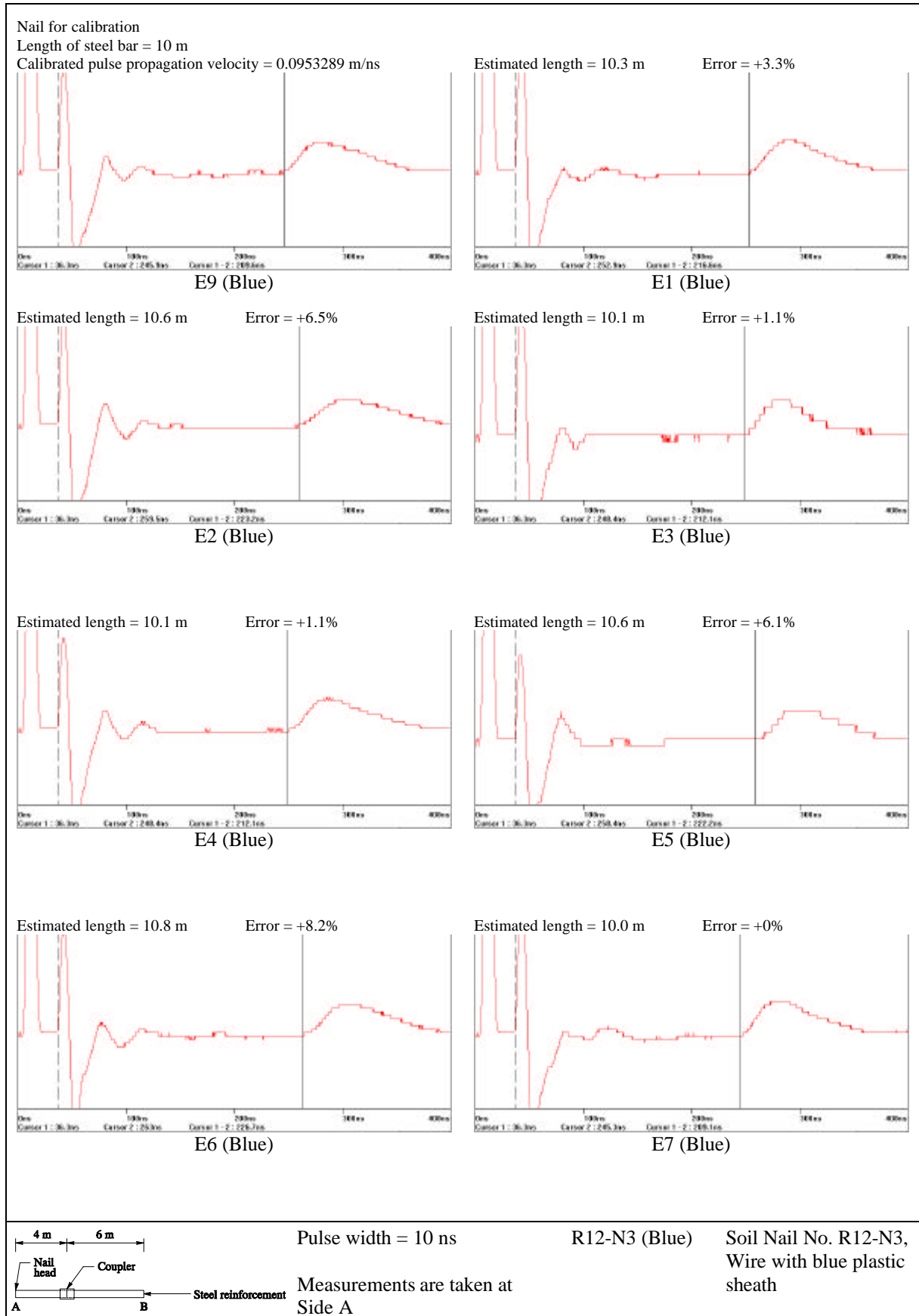
Figure 1 - TDR Test Results at an LPM Site in Chai Wan
