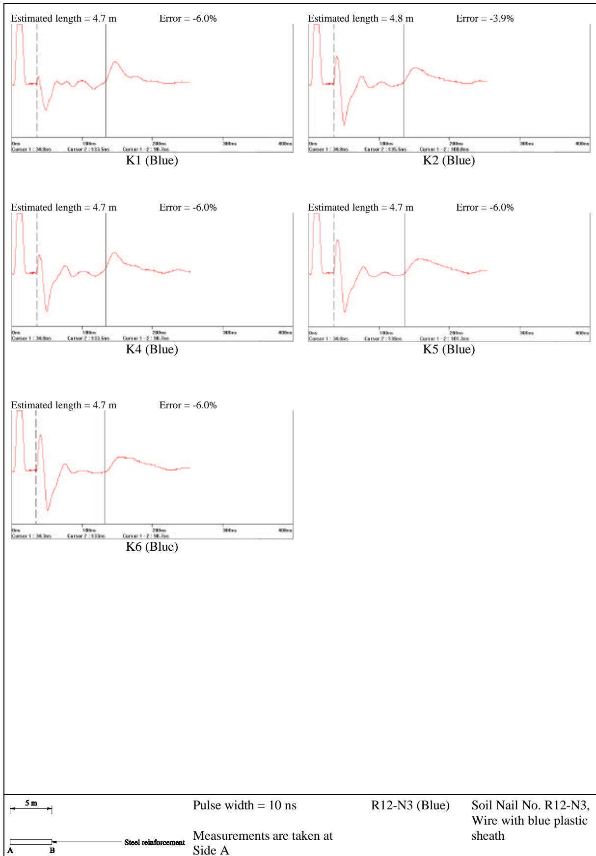
Figure 3 - TDR Test Results at an LPM Site in Chai Wan
