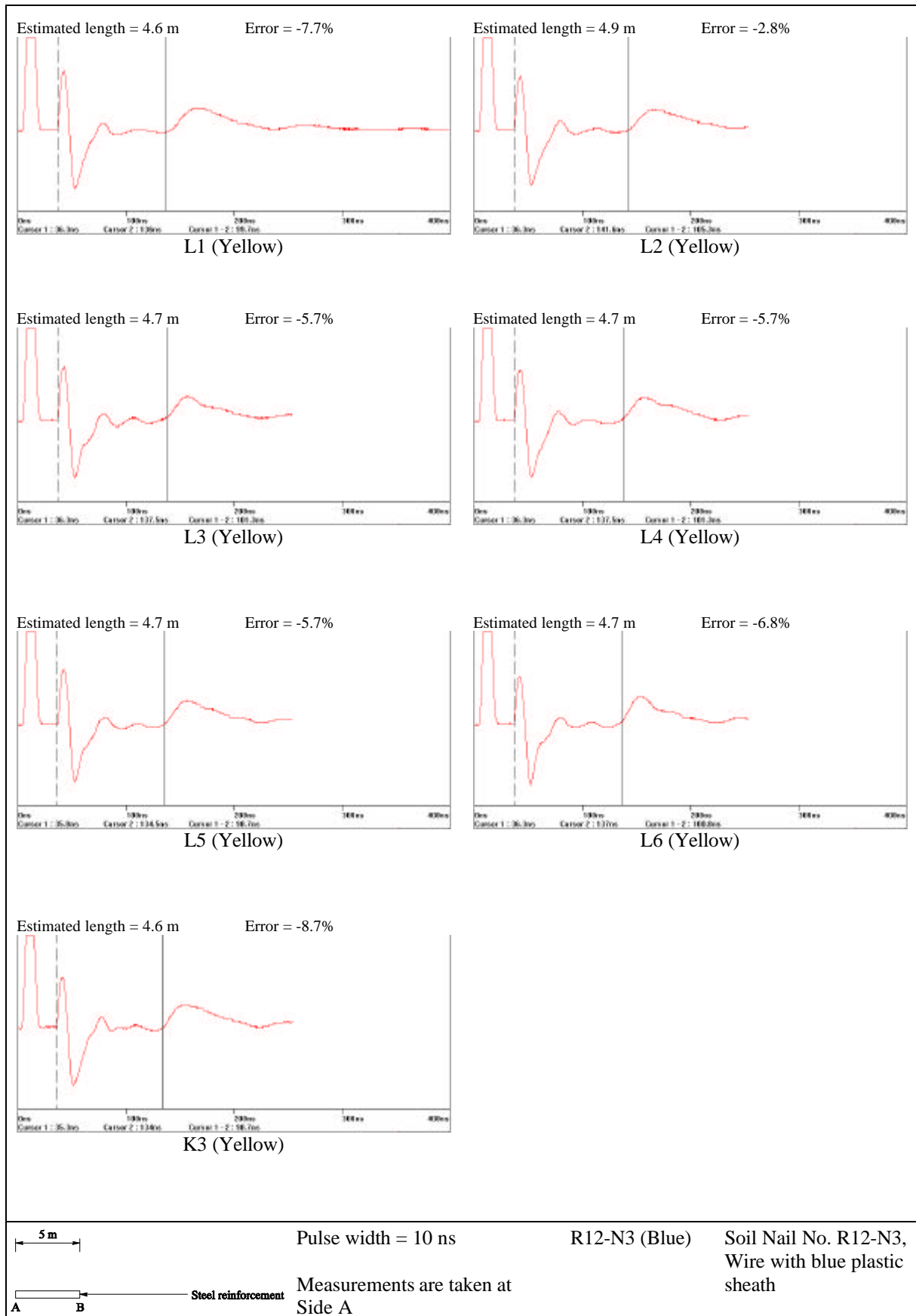
Figure 6 - TDR Test Results at an LPM Site in Chai Wan
