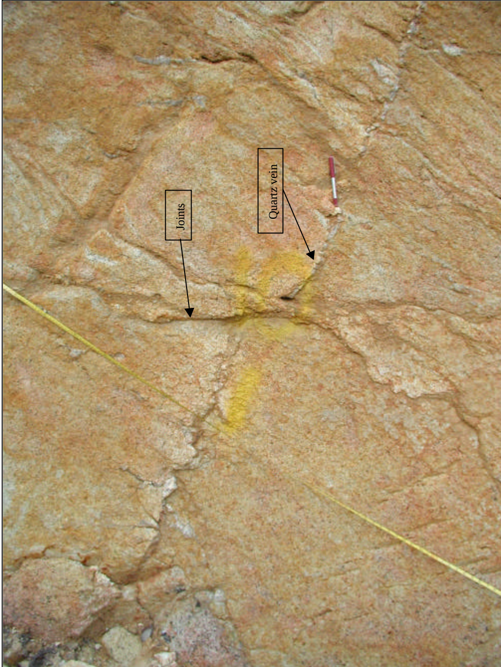
Plate 12 - Detail of Quartz Vein Offset by a Joint on the Eastern Flank of Landslide B (Photograph taken on 24 October 2000)
