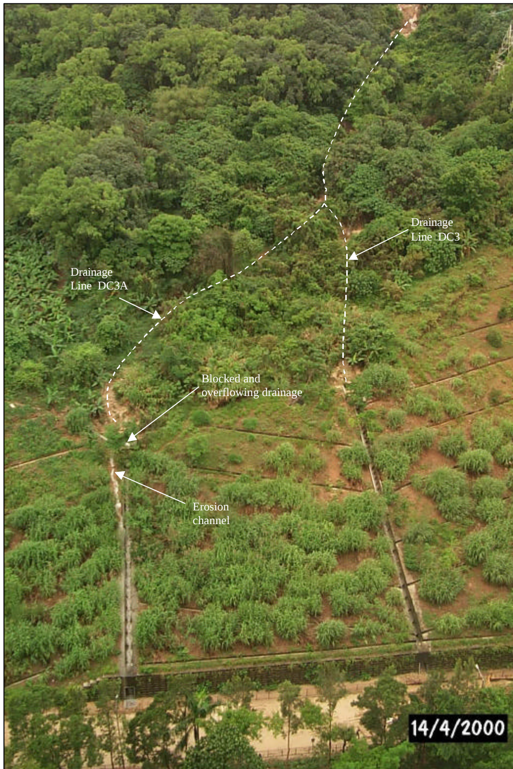
Plate 4 - View of the Blocked and Overflowing Slope Drainage Below the Source Area of Landslide B (Photograph taken by MCA on 14 April 2000)
