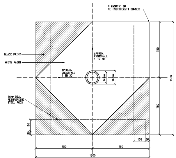
BEDROCK BENCHMARK PLAN VIEW
