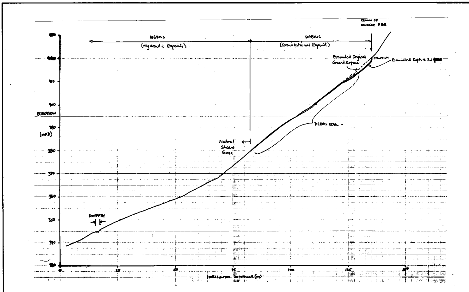
Figure A23 - Cross-section of Landslide A16B
