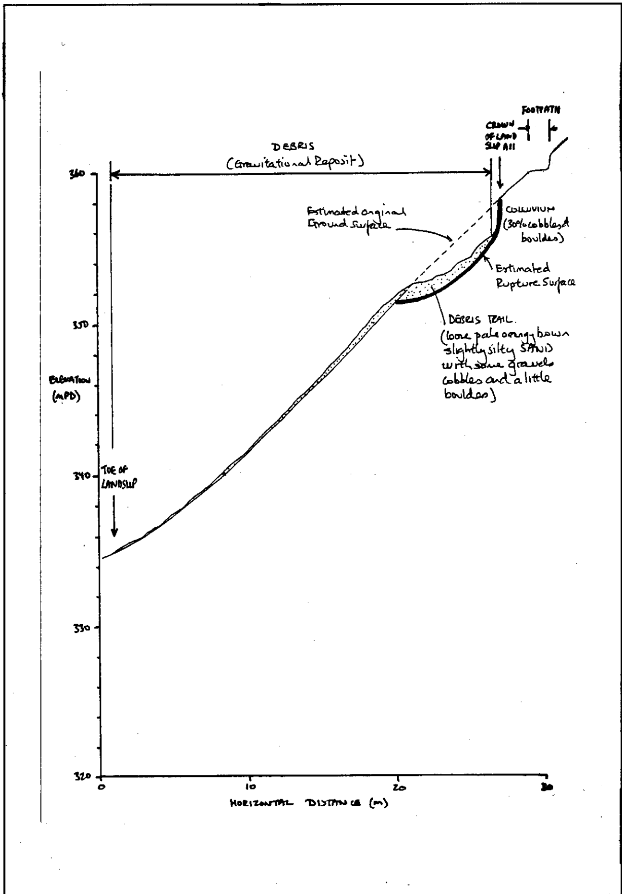
Figure A16 - Cross-section of Landslide A11
