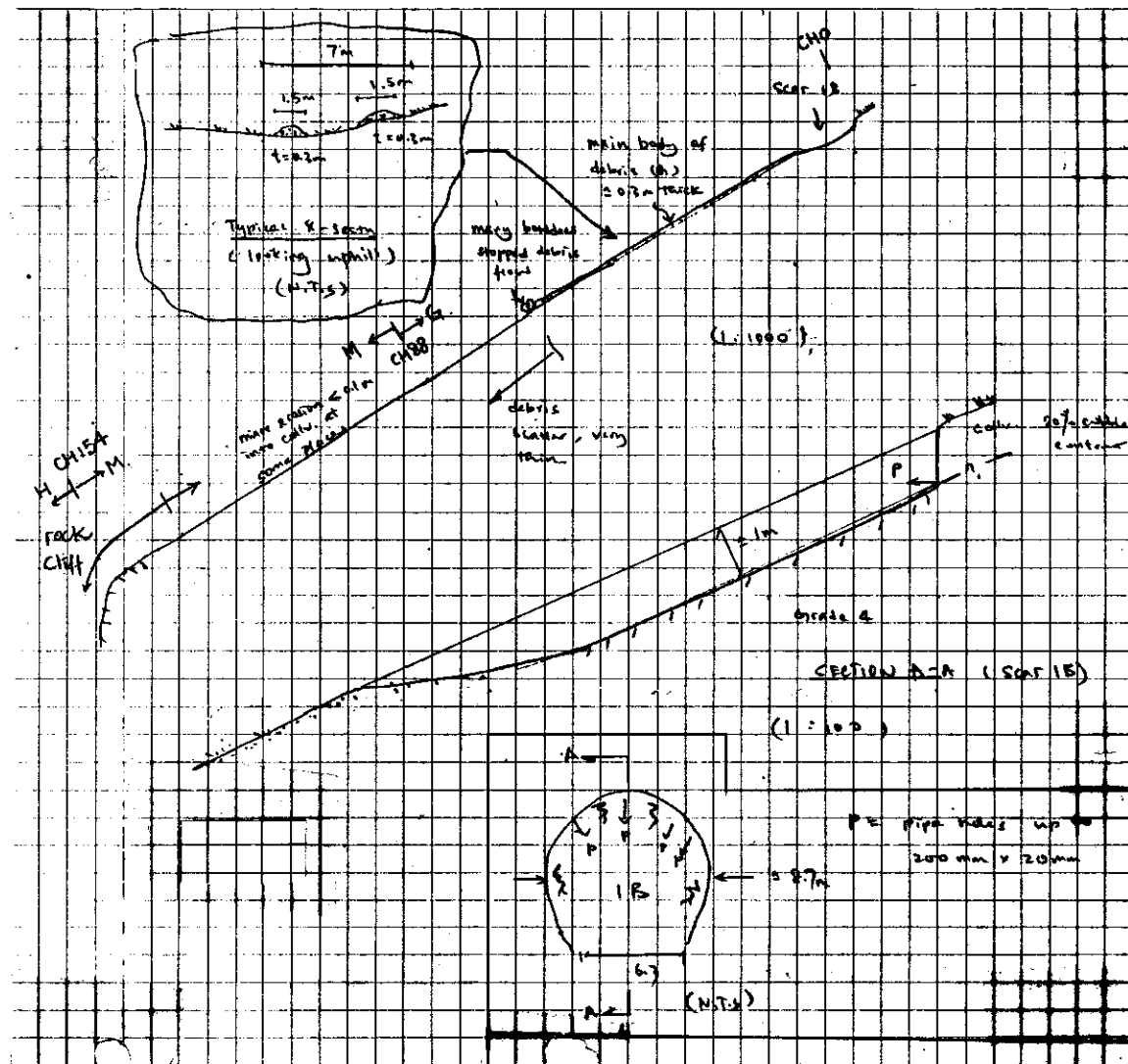
Figure A1 - Cross-section of Landslide A1A
