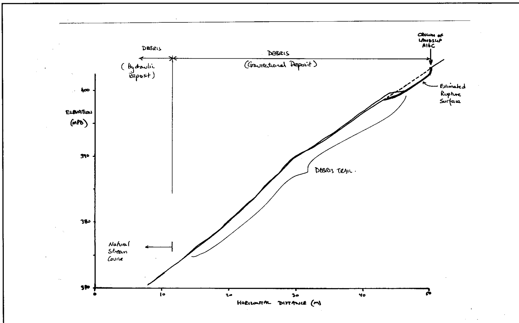
Figure A24 - Cross-section of Landslide A16C
