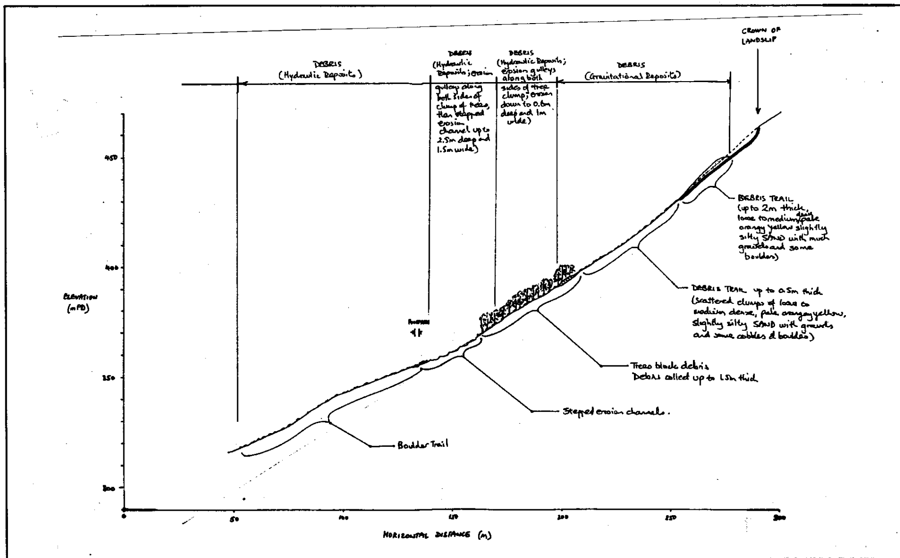
Figure A25 - Cross-section of Landslide A17
