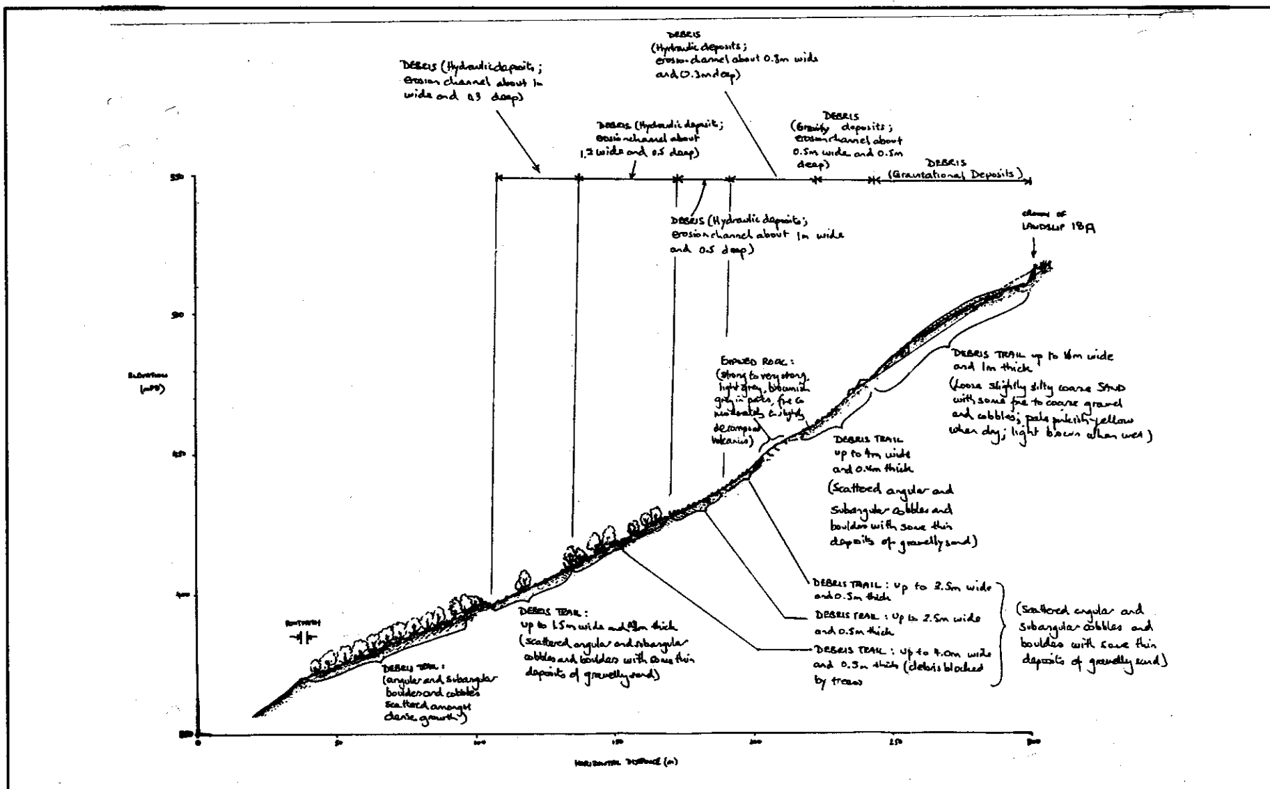
Figure A26 - Cross-section of Landslide A18A
