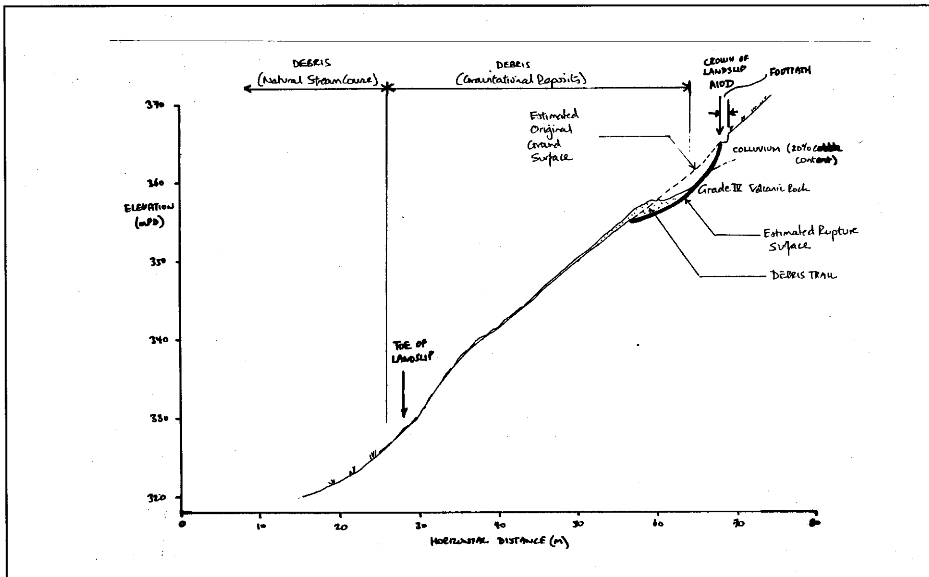
Figure A15 - Cross-section of Landslide A10D
