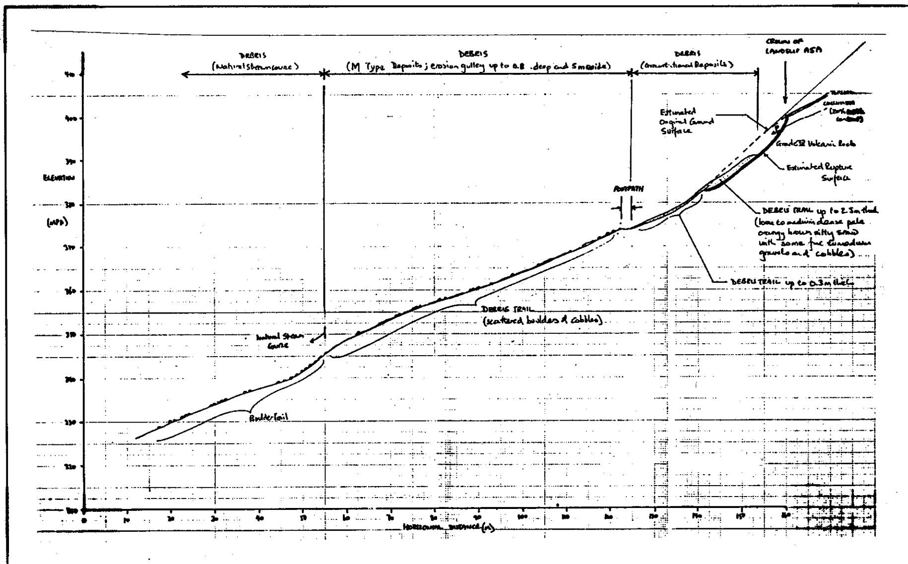
Figure A6 - Cross-section of Landslide A5A
