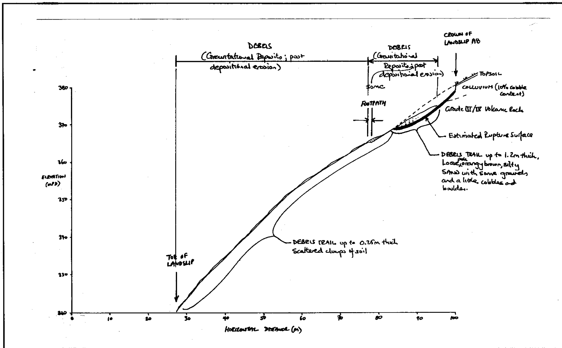
Figure A10 - Cross-section of Landslide A8
