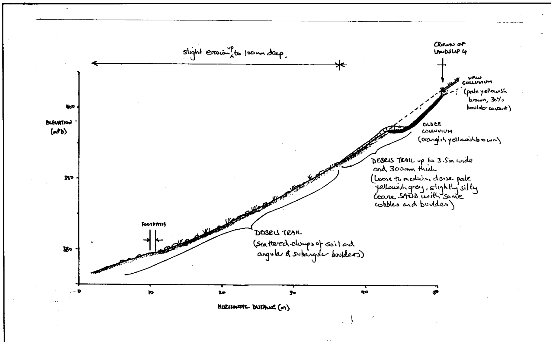
Figure A5 - Cross-section of Landslide A4
