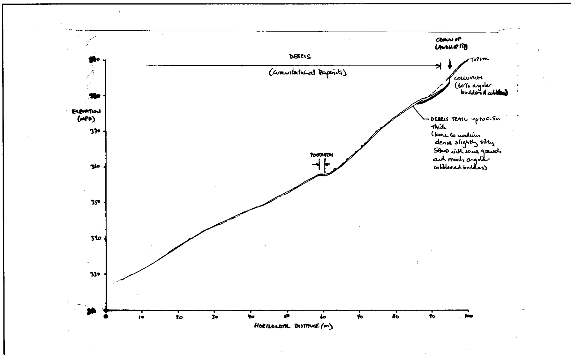
Figure A19 - Cross-section of Landslide A13B
