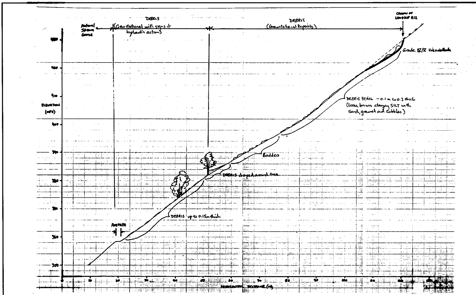
Figure A17 - Cross-section of Landslide A12
