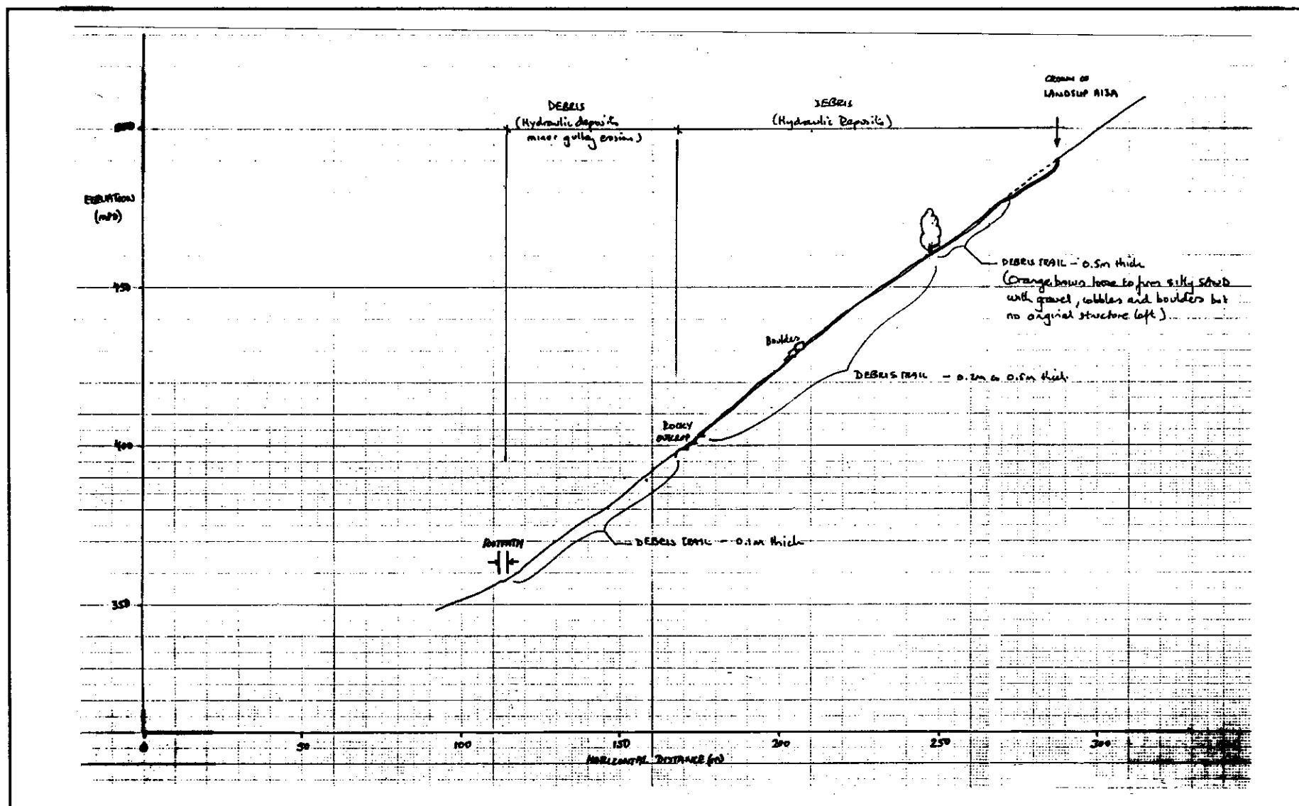
Figure A18 - Cross-section of Landslide A13A
