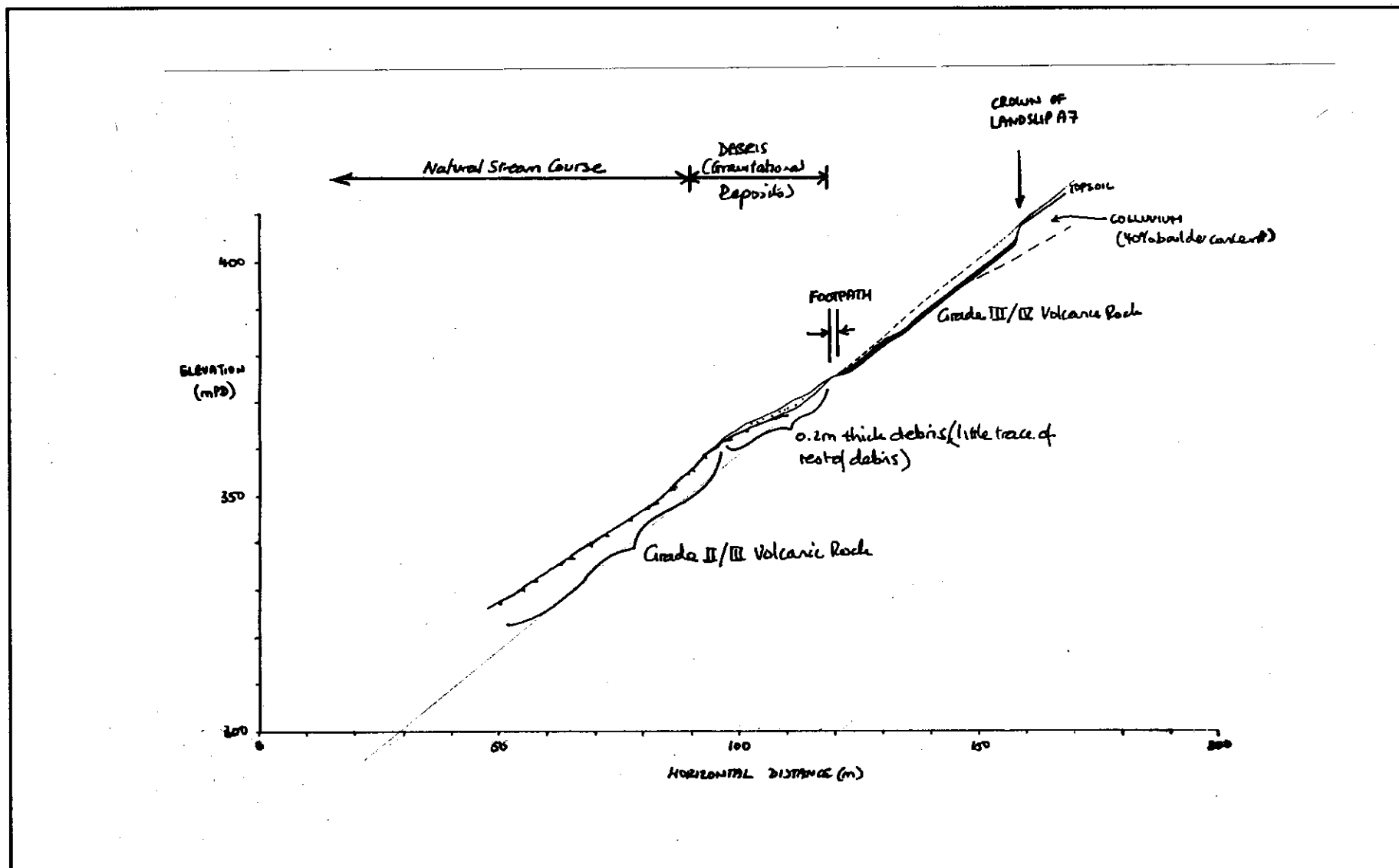
Figure A9 - Cross-section of Landslide A7
