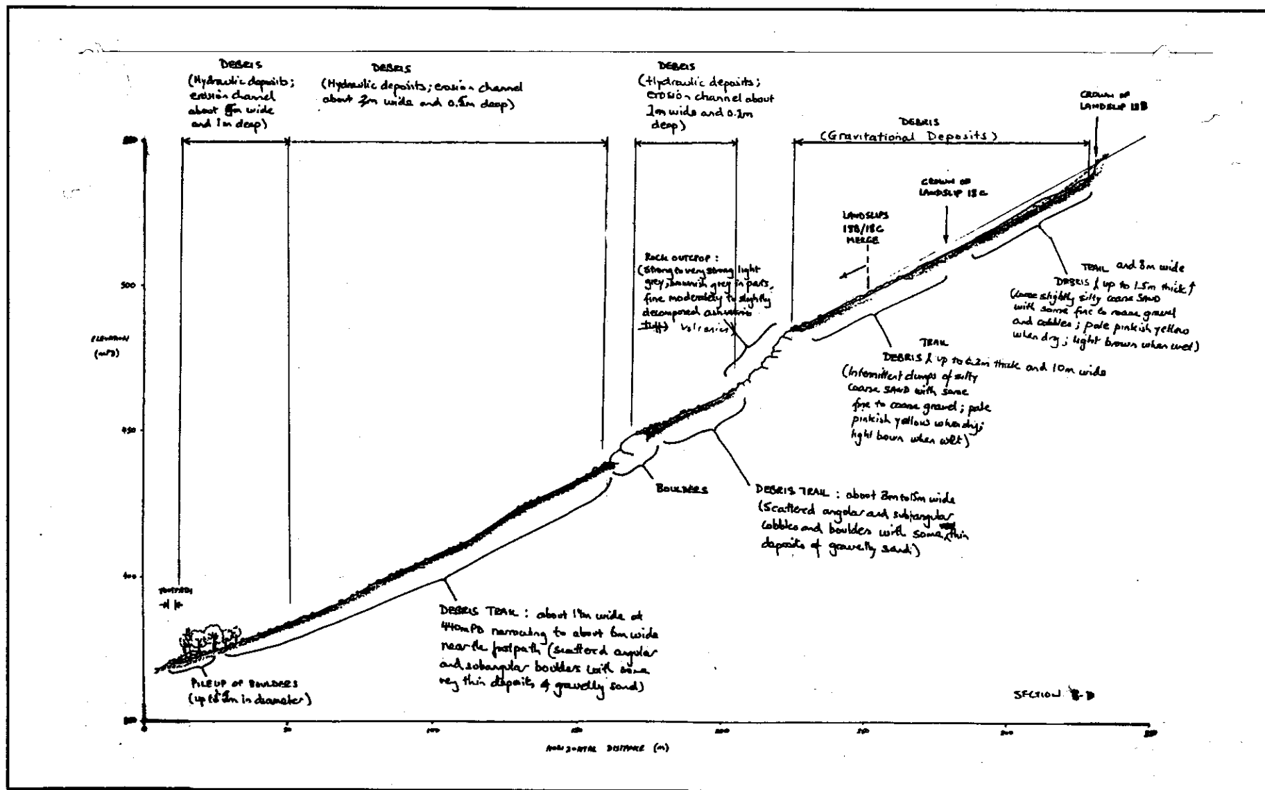
Figure A27 - Cross-section of Landslide A18B
