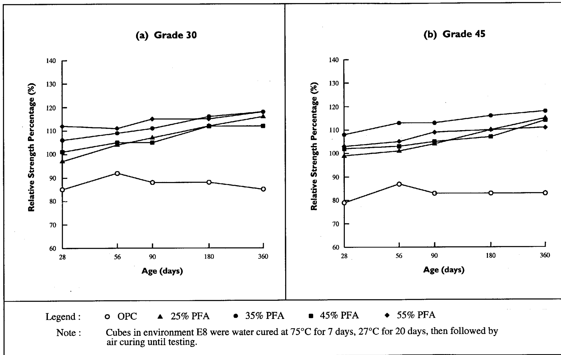
Figure 7 - Influence of High Initial Curing Temperature (Environment E8) on the Strength Development of OPC and PFA Concretes
