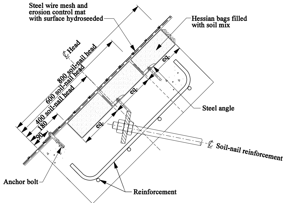
Typical Section
