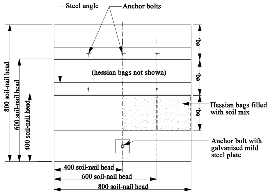
Typical Elevation
