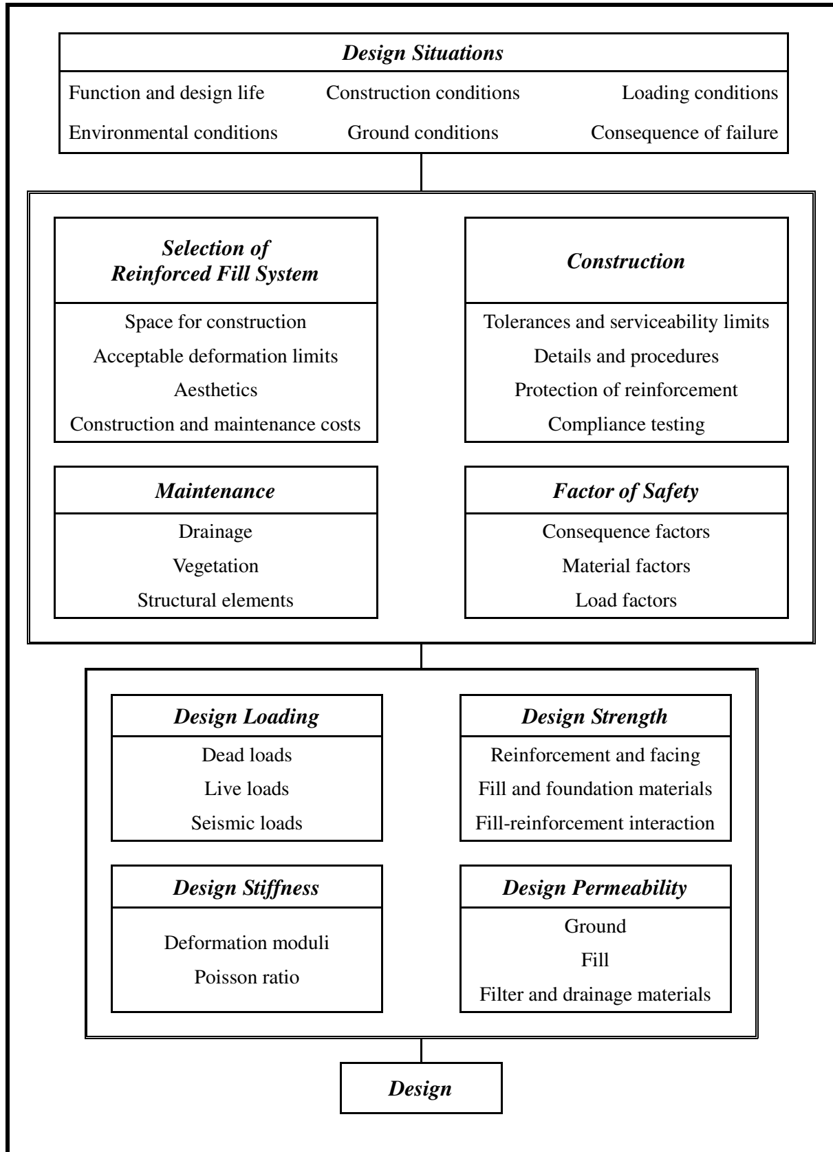
Figure 27 – Design Considerations for Reinforced Fill Structures and Slopes
