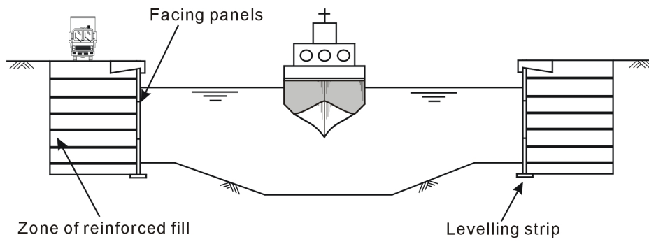
(a) River Training Structures
