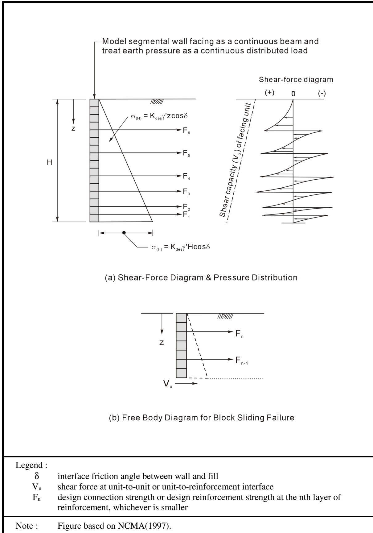
Figure 49 – Analysis of Block Sliding Failure of Segmental Block Wall
