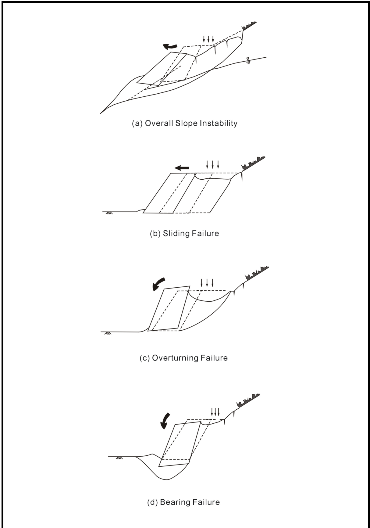
Figure 28 – Ultimate Limit States - External Instability
