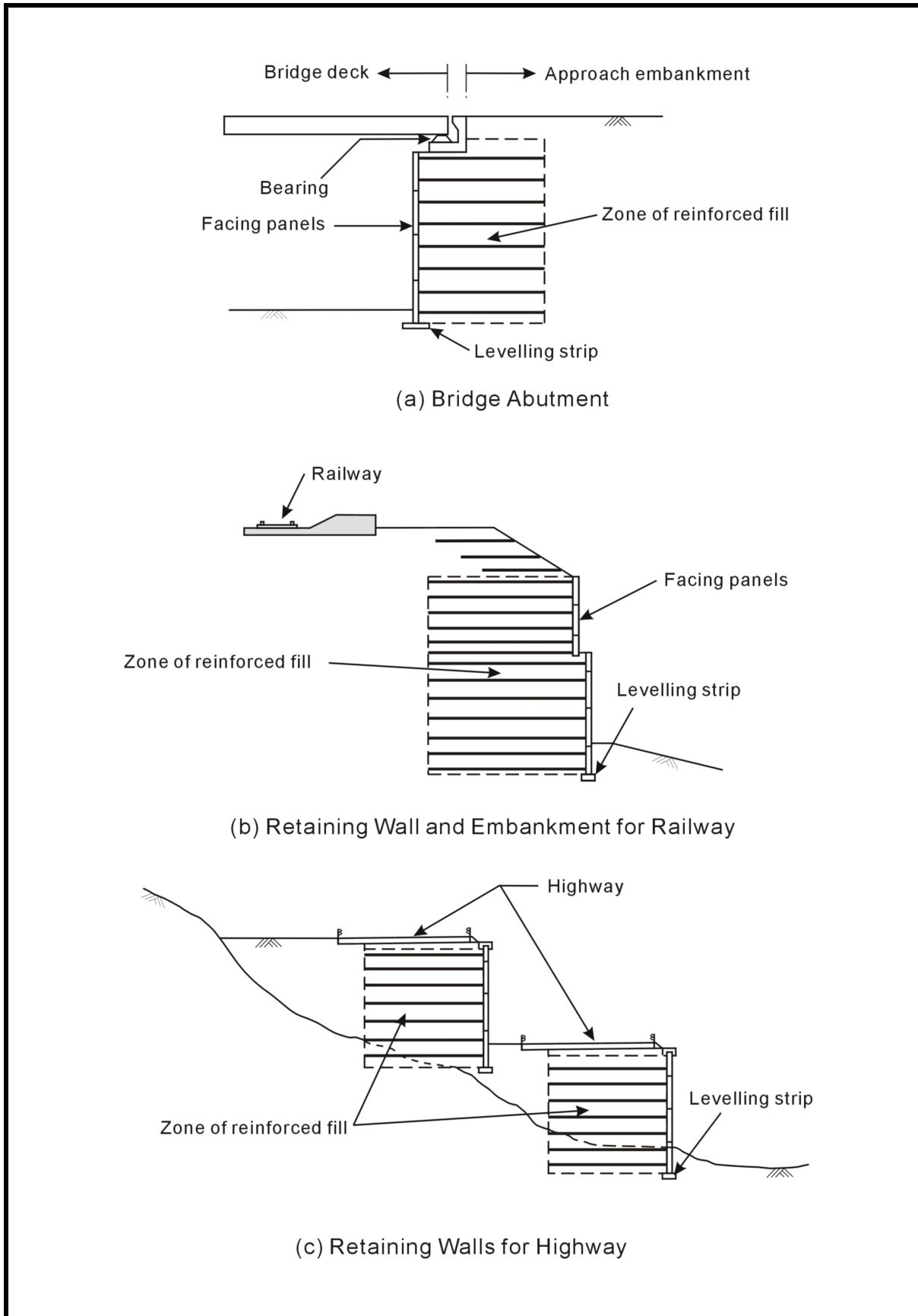
Figure 2 – The Use of Reinforced Fill in Highway and Railway Application
