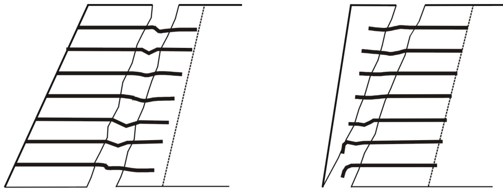
(b) Pullout of Reinforcement from the Yielding Fill Mass (Front Face Pullout)
