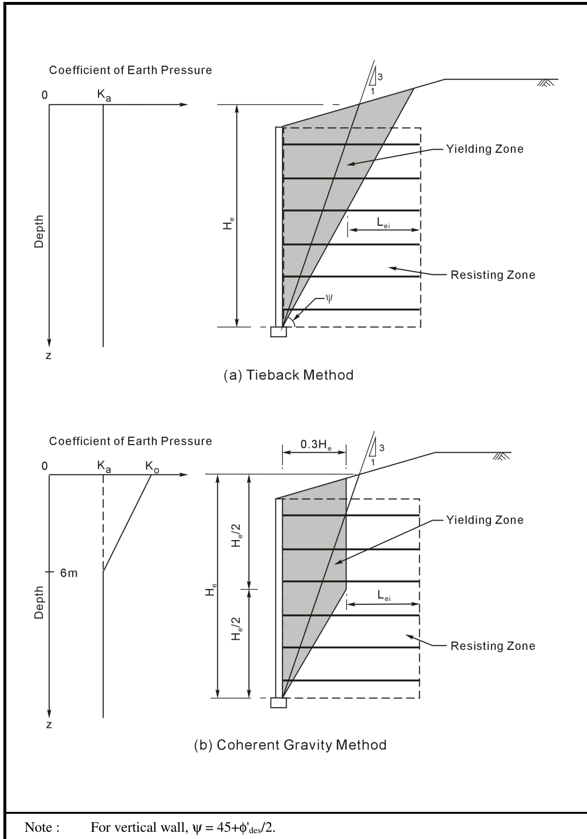
Figure 36 – Design Methods for Internal Stability Analysis of Reinforced Fill Structures
