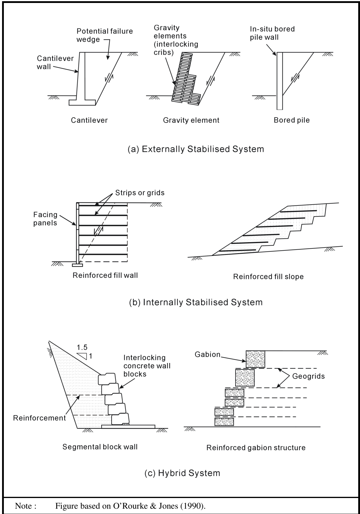
Figure 13 – Classification of Common Earth Retention Systems
