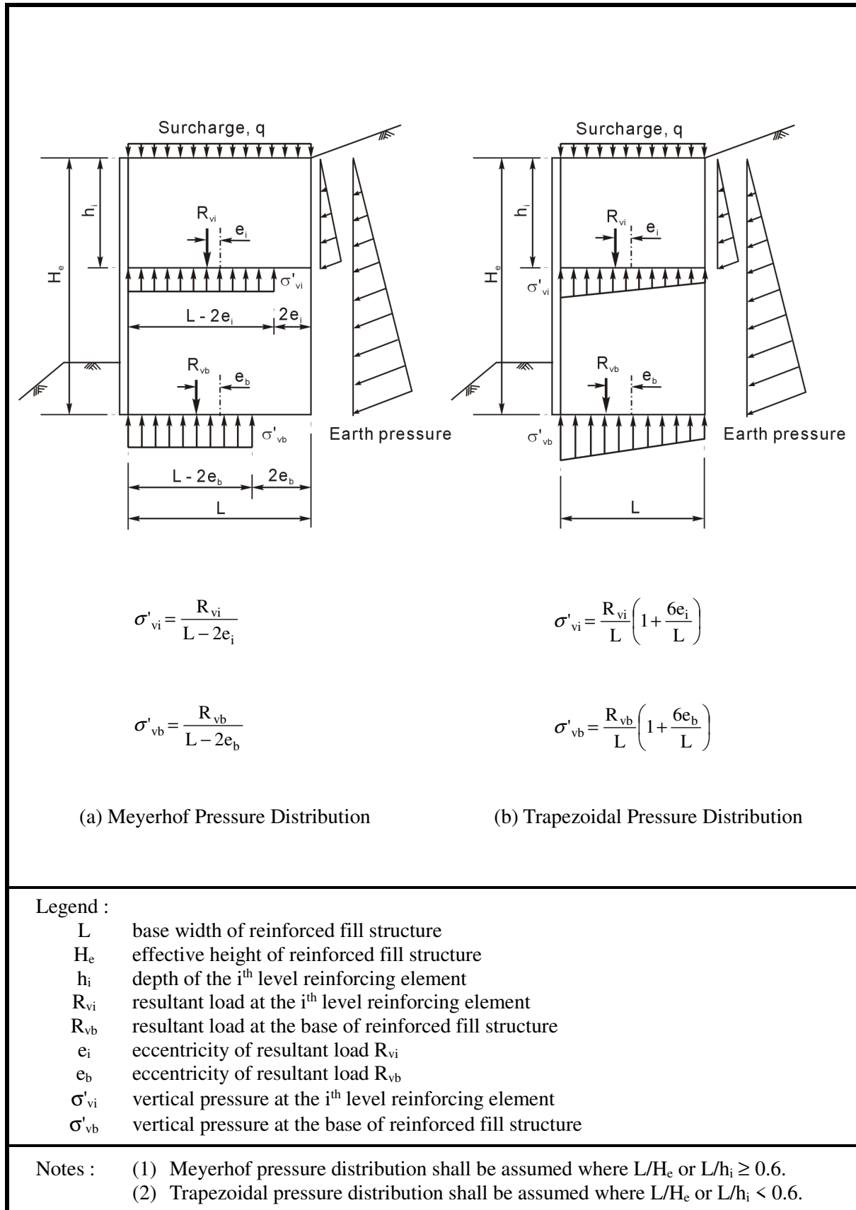
Figure 35 – Stresses Imposed due to Self Weight, Surcharge and Retained Backfill
