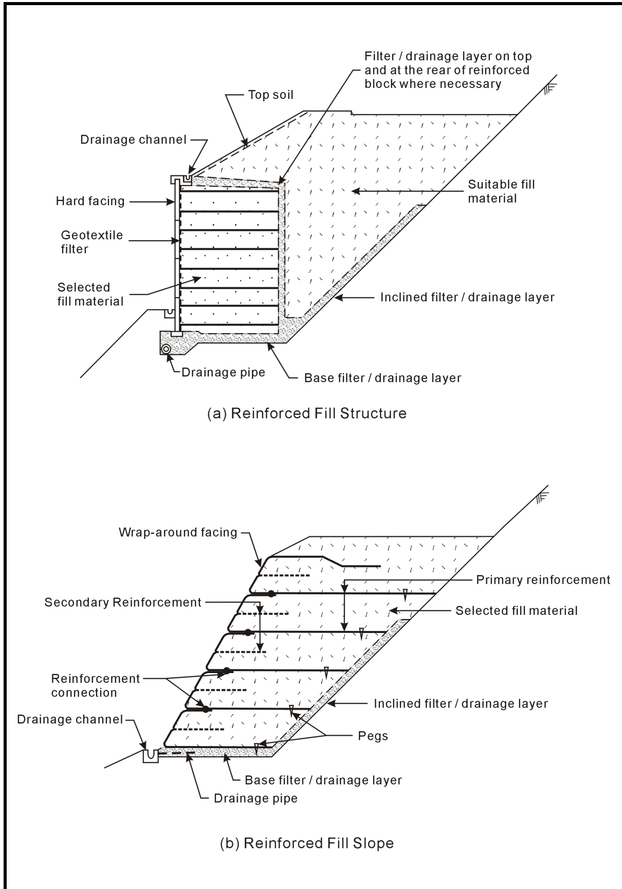
Figure 43 – Typical Drainage Layouts for Reinforced Fill Structures and Slopes
