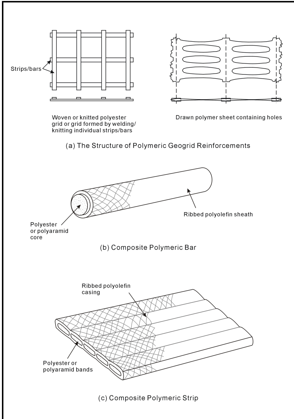
Figure 23 – Polymeric Reinforcement
