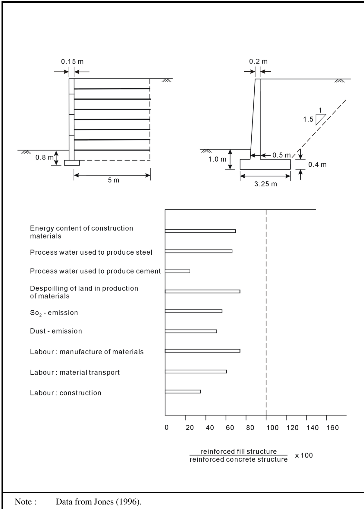
Figure 7 – Ecological Parameters for a 6 m High Reinforced Fill Structure and an Equivalent Reinforced Concrete Structure
