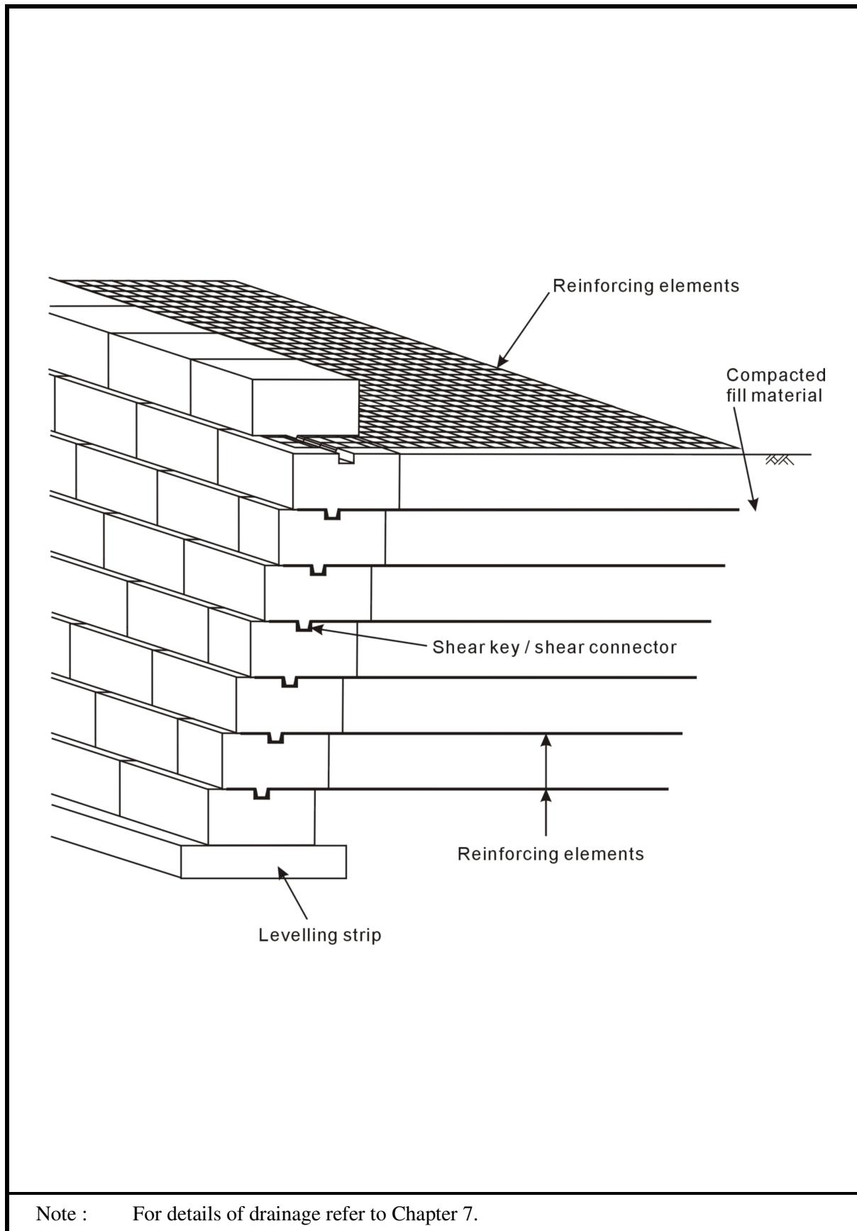
Figure 11 – Segmental Block System
