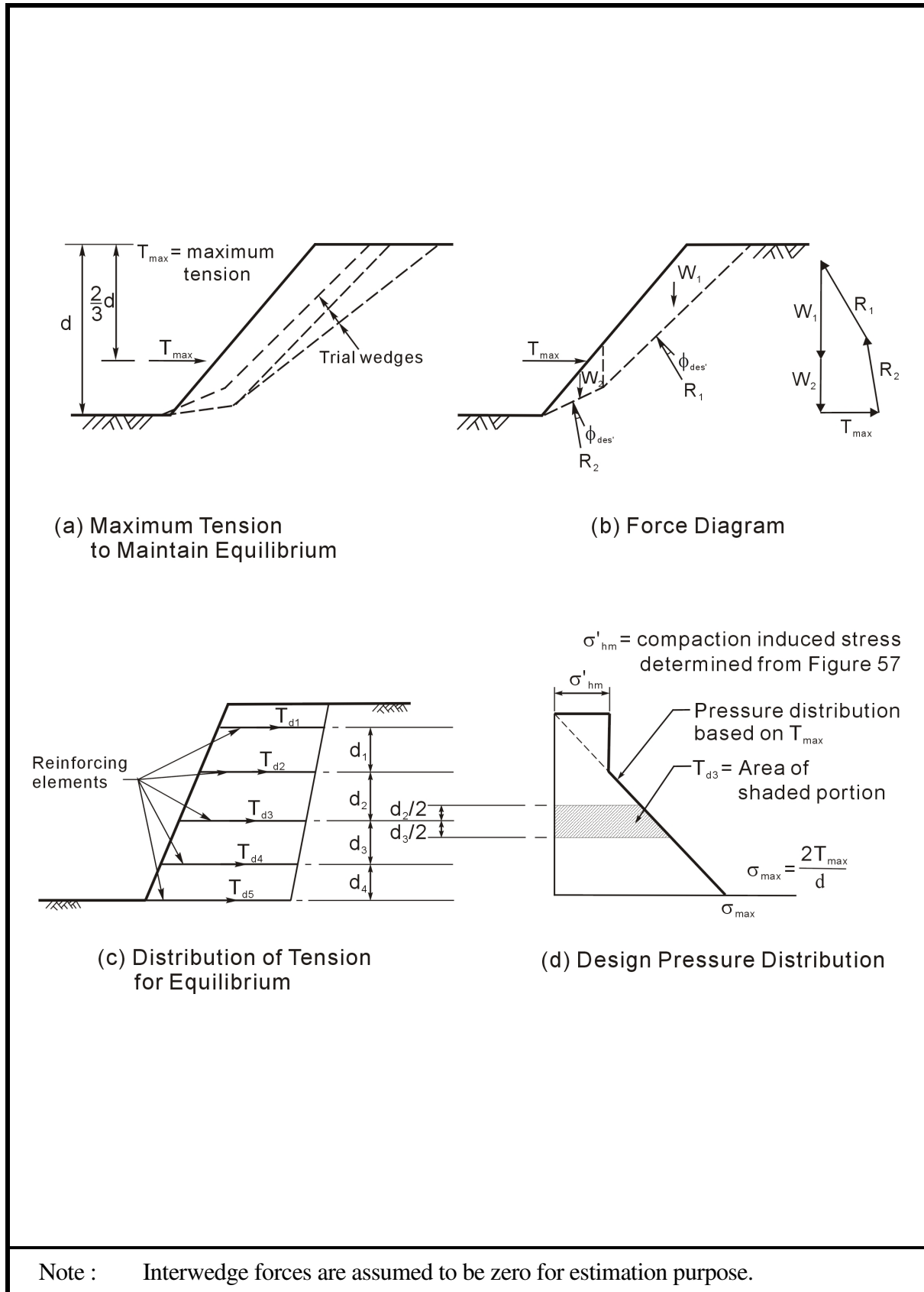
Figure 59 – Estimation of the Design Tension by Two-part Wedge Method
