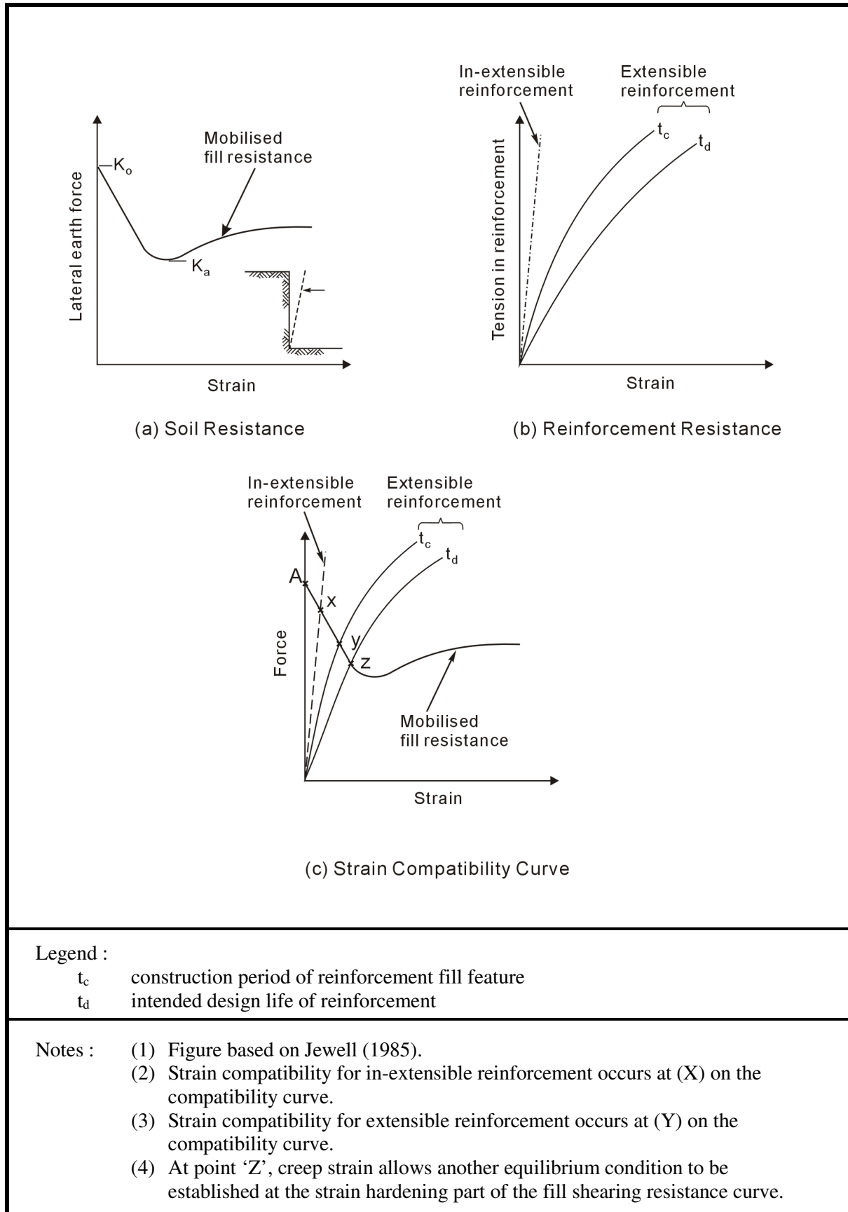
Figure 16 – Condition of Strain Compatibility
