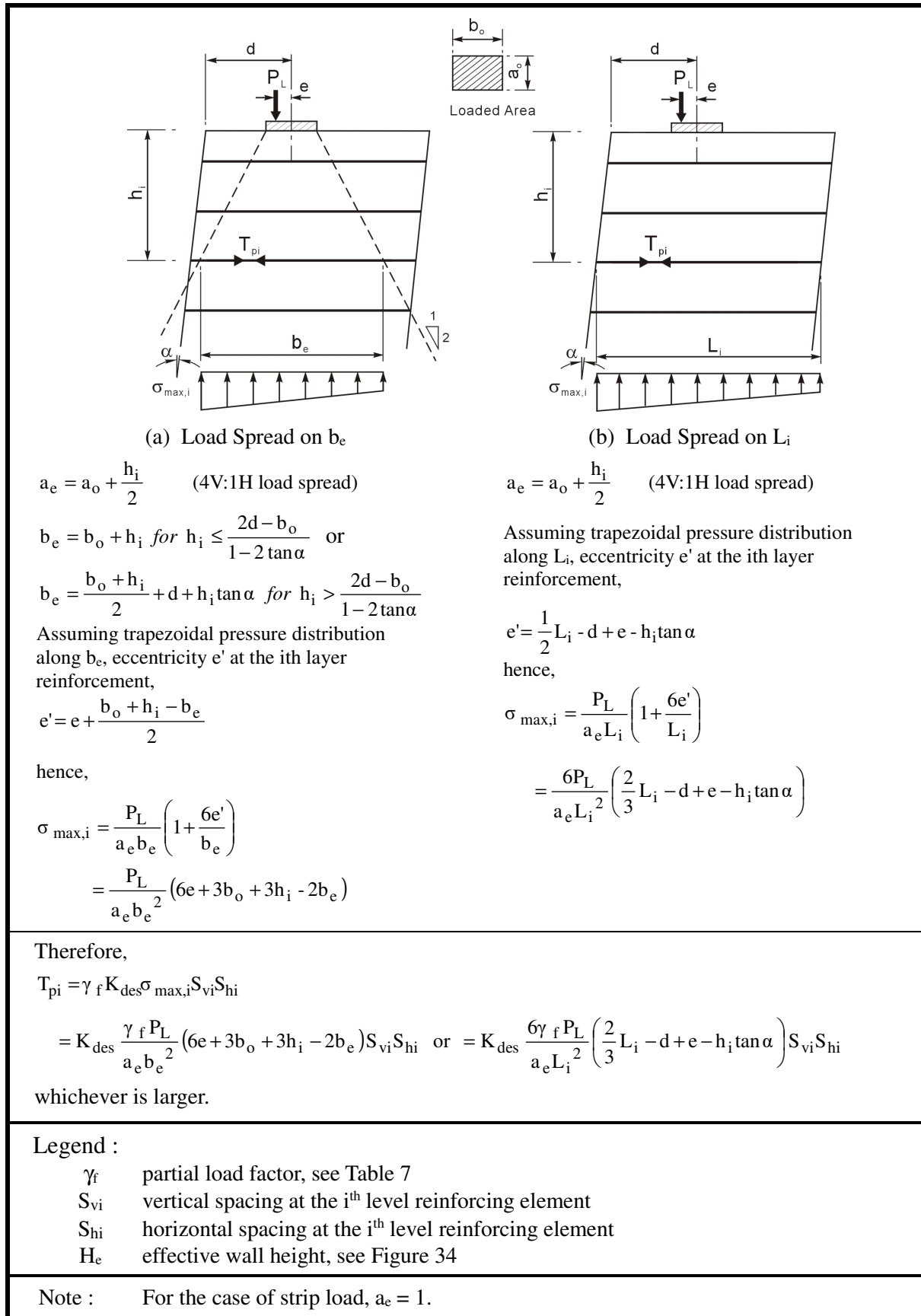
Figure 37 – Tensile Force due to Vertical Load P_L on Top of the Structure
