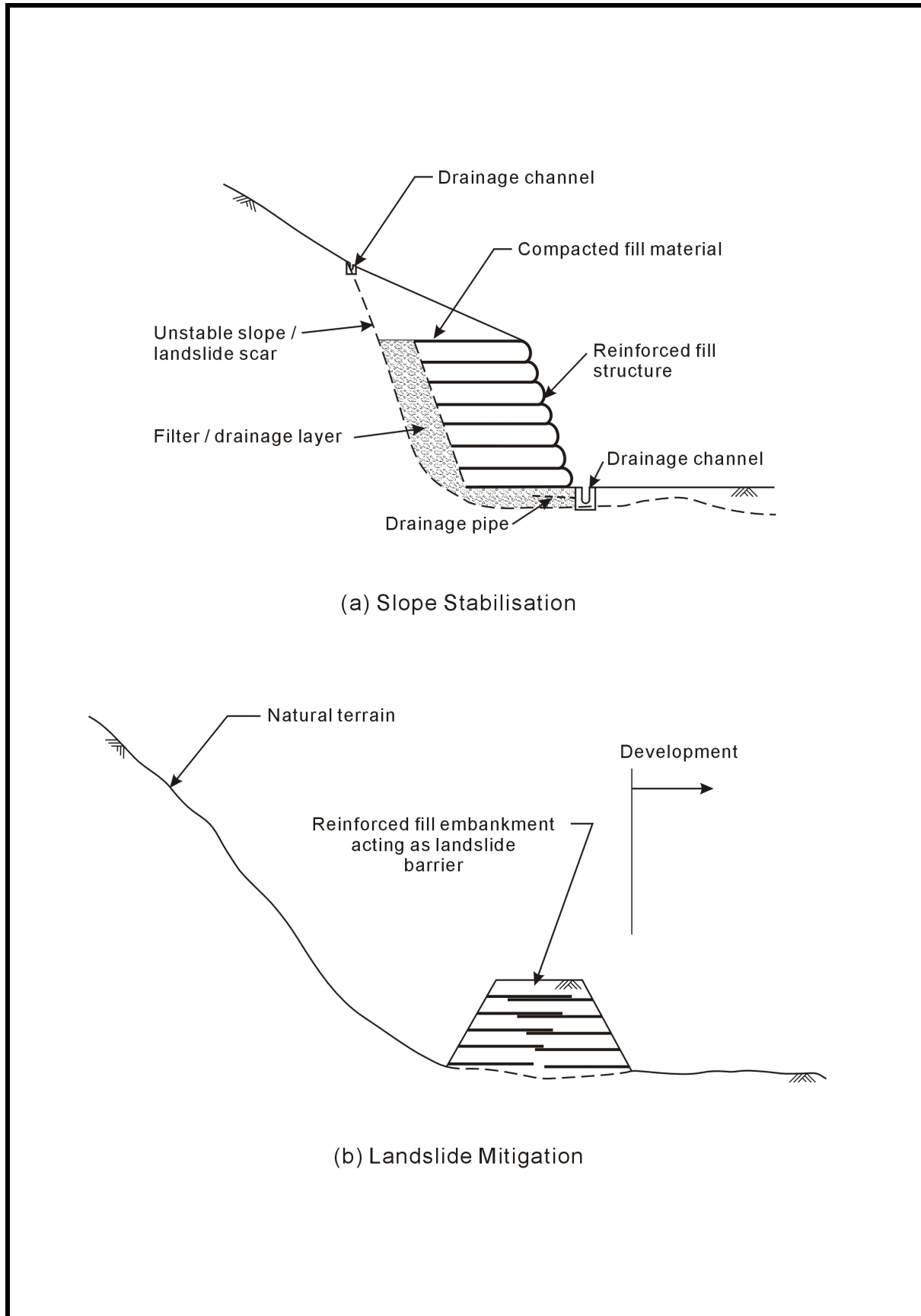
Figure 4 – The Use of Reinforced Fill in Slope Stabilization and Landslide Mitigation
