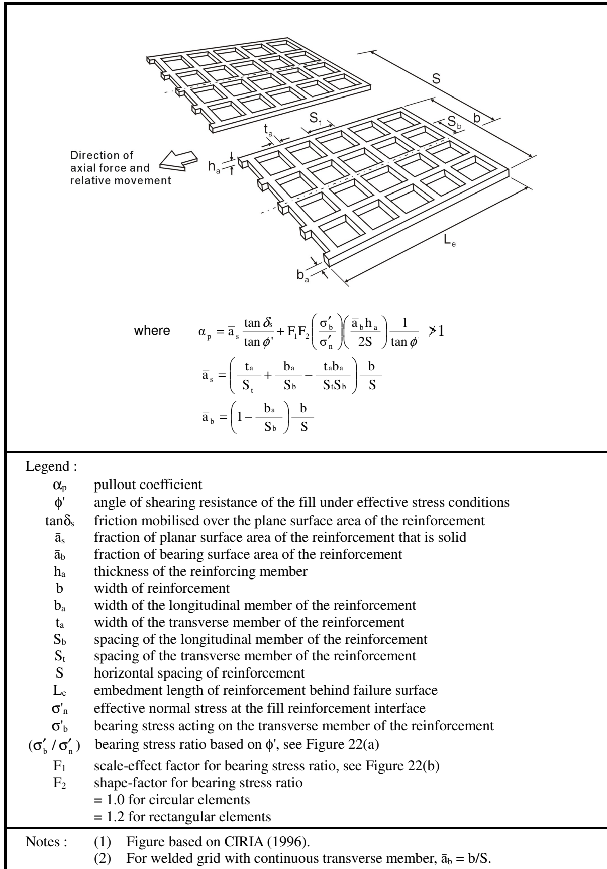
Figure 20 – Pullout Resistance of Grid Reinforcement
