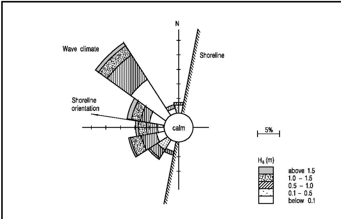
Figure 8 - Wave Rose
