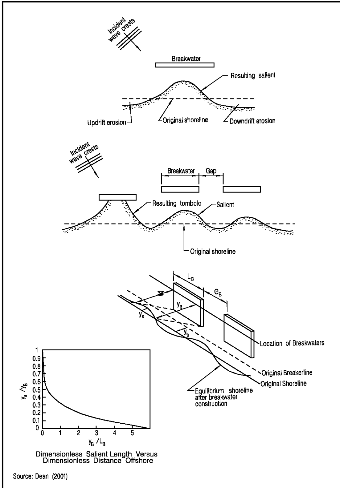
Figure 14 – Detached Breakwaters
