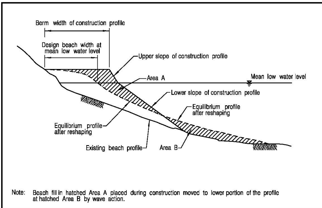
Figure 9 - Construction Profile
