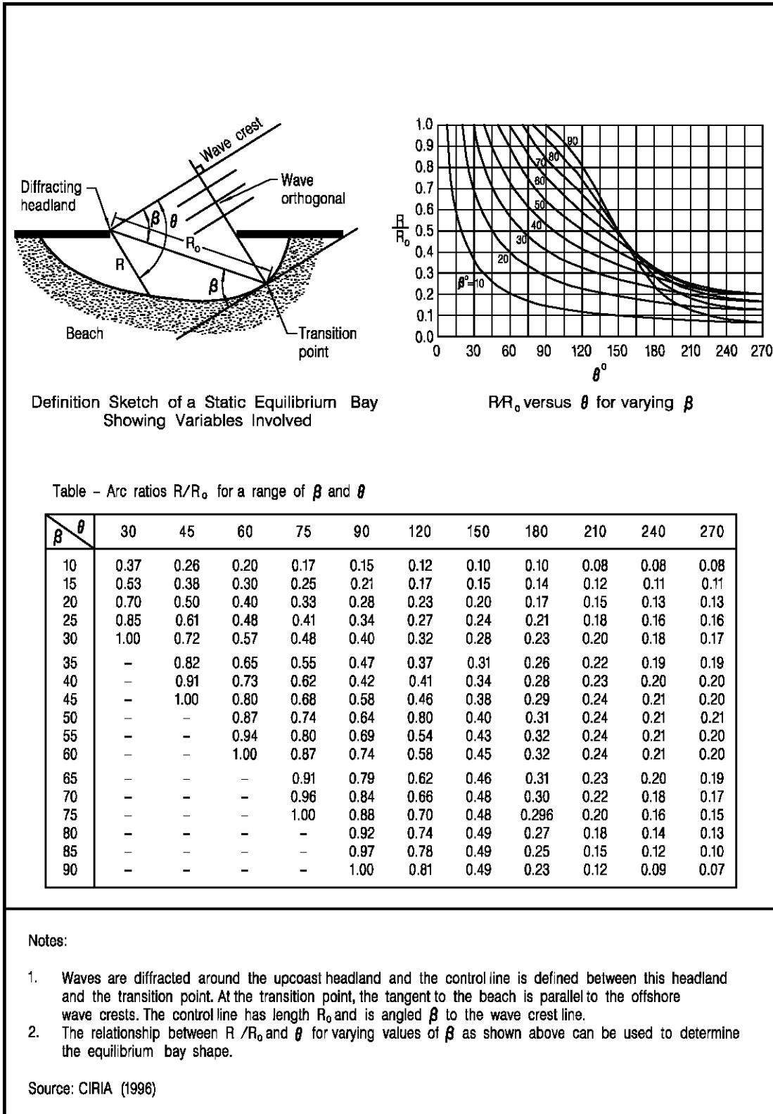
Figure 15 – Artificial Headlands
