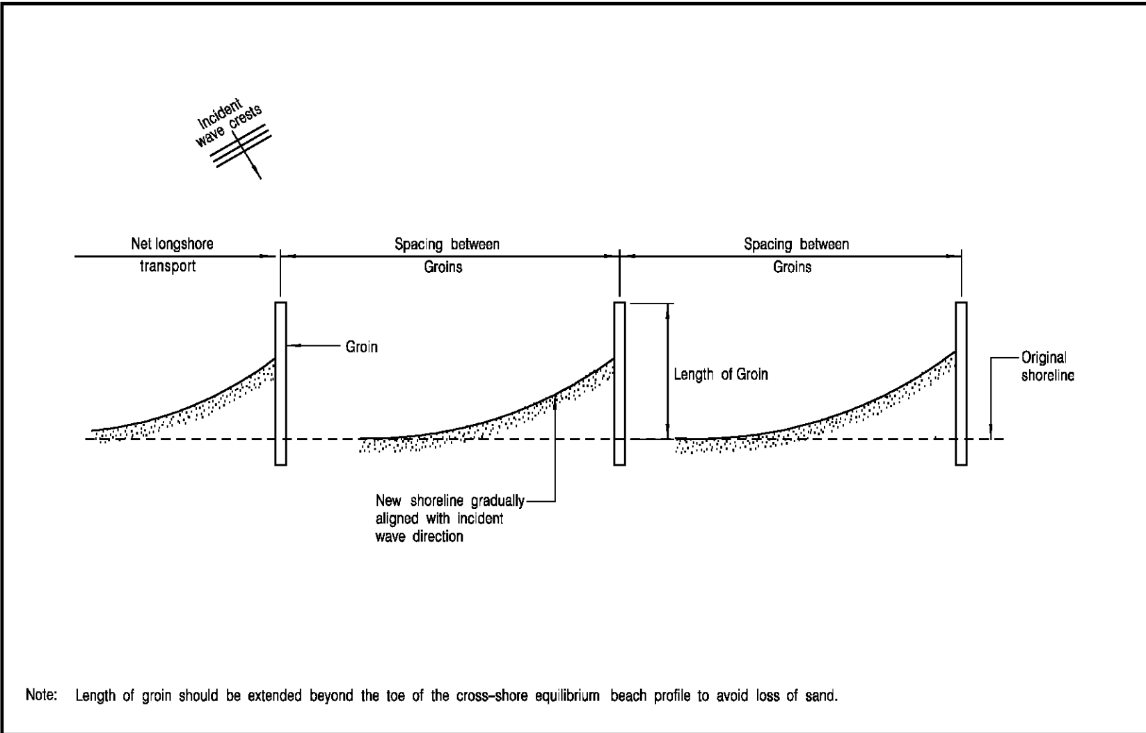
Figure 13 – Groins
